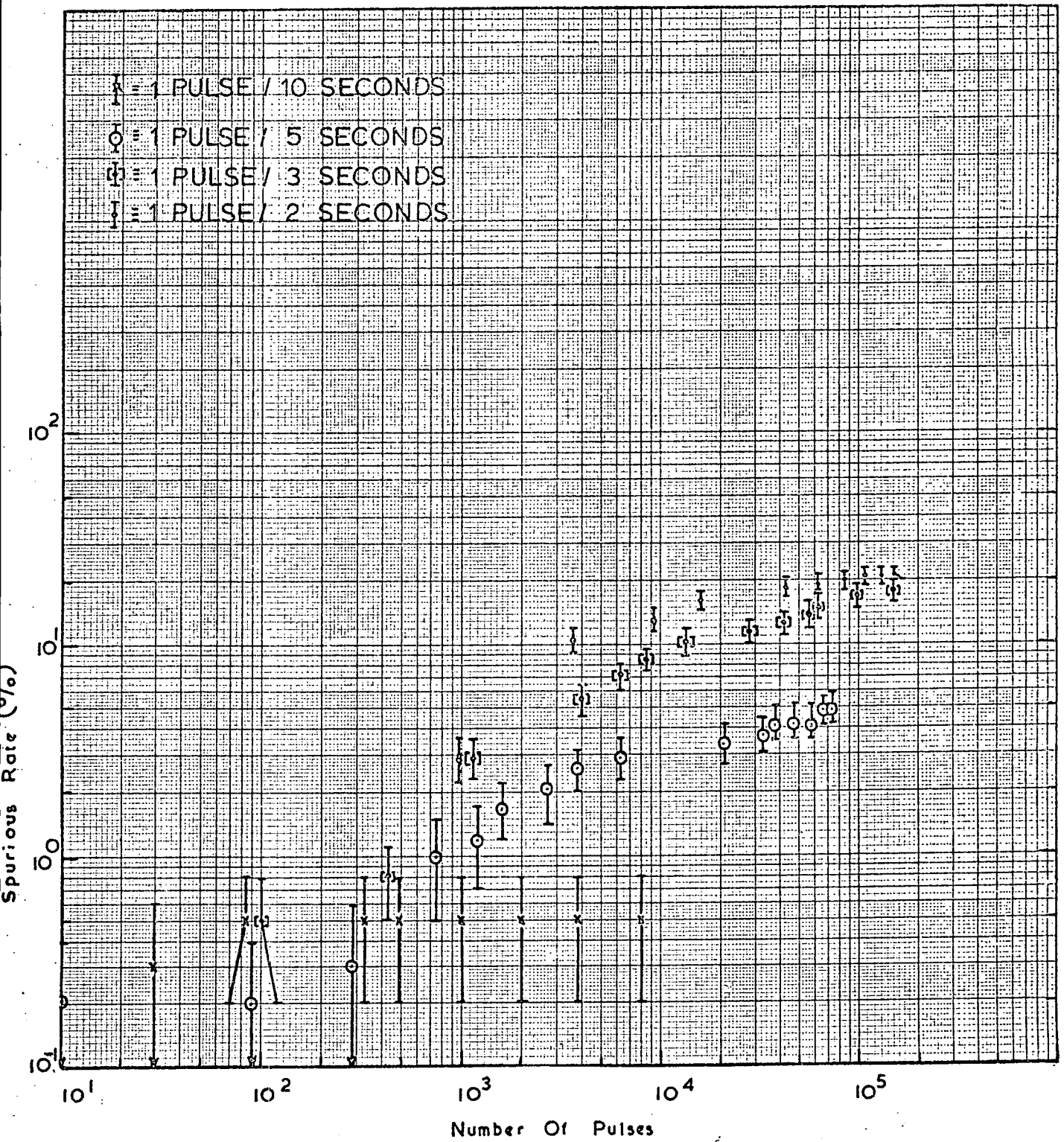
Figure B.1 Graphs of the Spurious Rate against Number of Pulses for Various Pulsing Rates.
