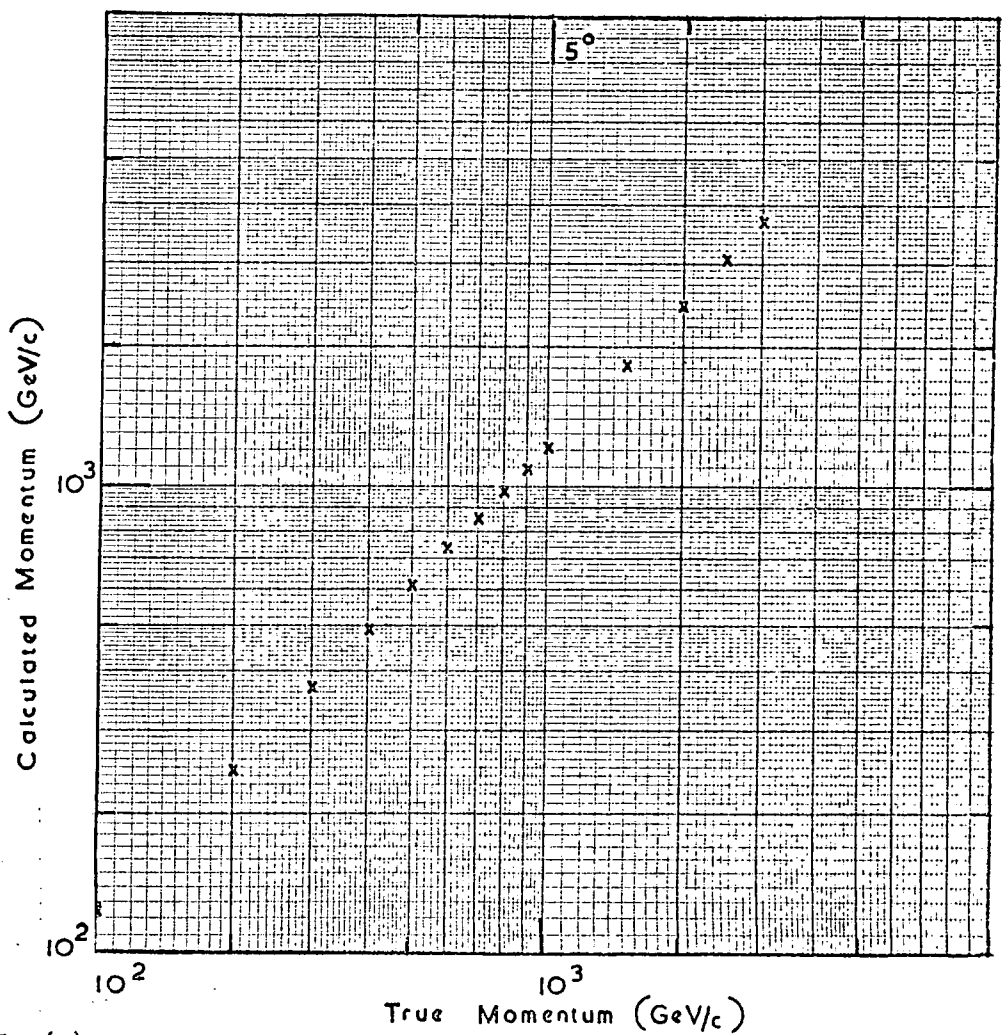
Figure 7.5(b) Graph of Calculated Momentum against True Momentum for an Incident Angle of 5°.
