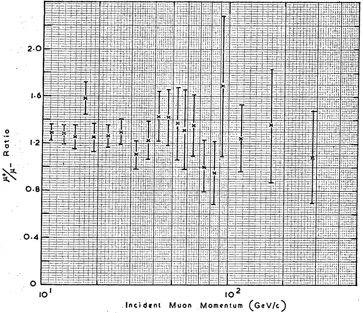
Figure 8.3 The Variation in the Muon Charge Ratio with Momentum from the results of the Preliminary Experiment.
