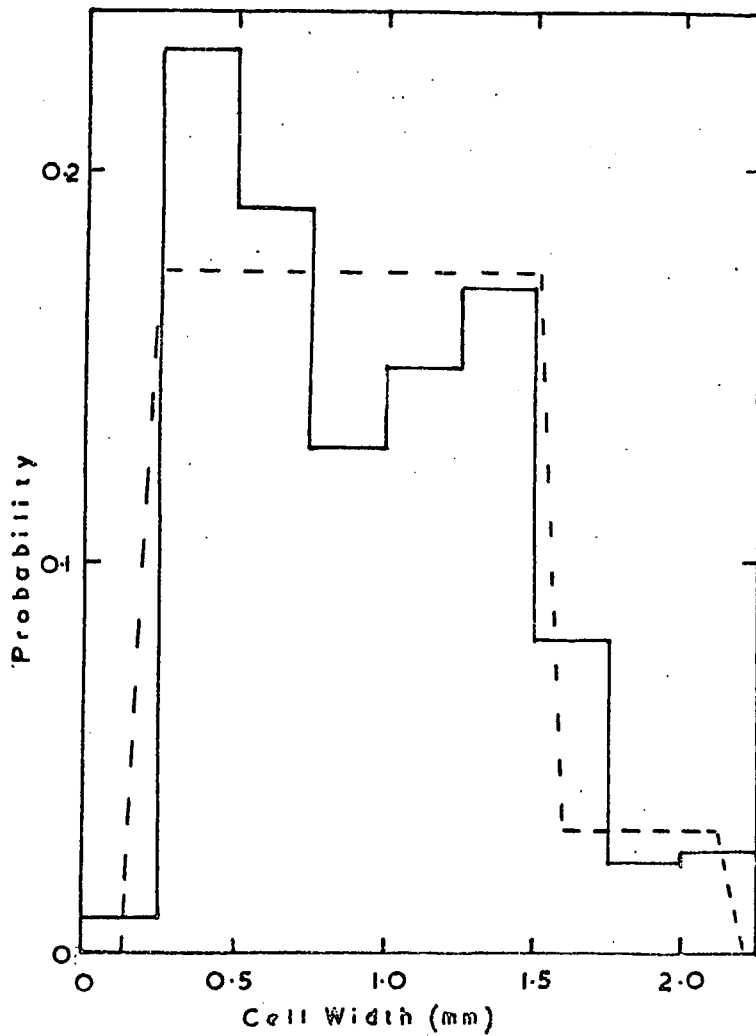
Figure 7.7 Probability Distribution of the Weighted Cell Widths.
