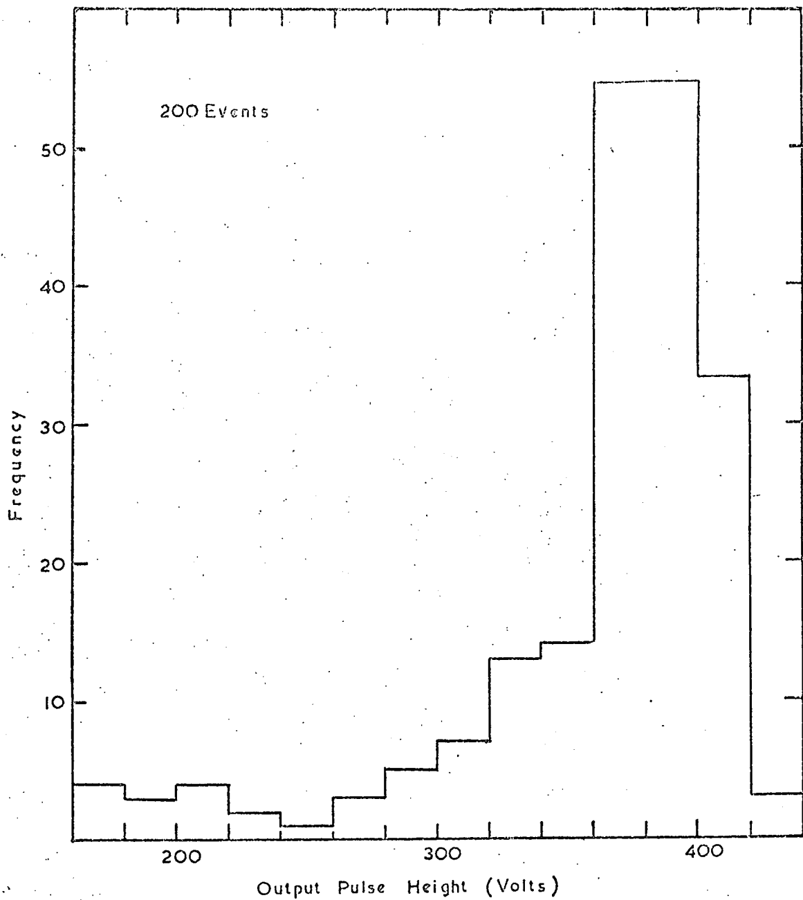
Figure 4.6 Histogram of the Pulse Height of 200 Events.
