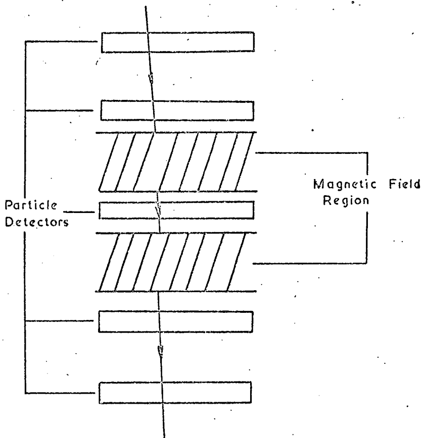
Figure 2.3 Schematic Form of a Multilayer Spectrograph.
