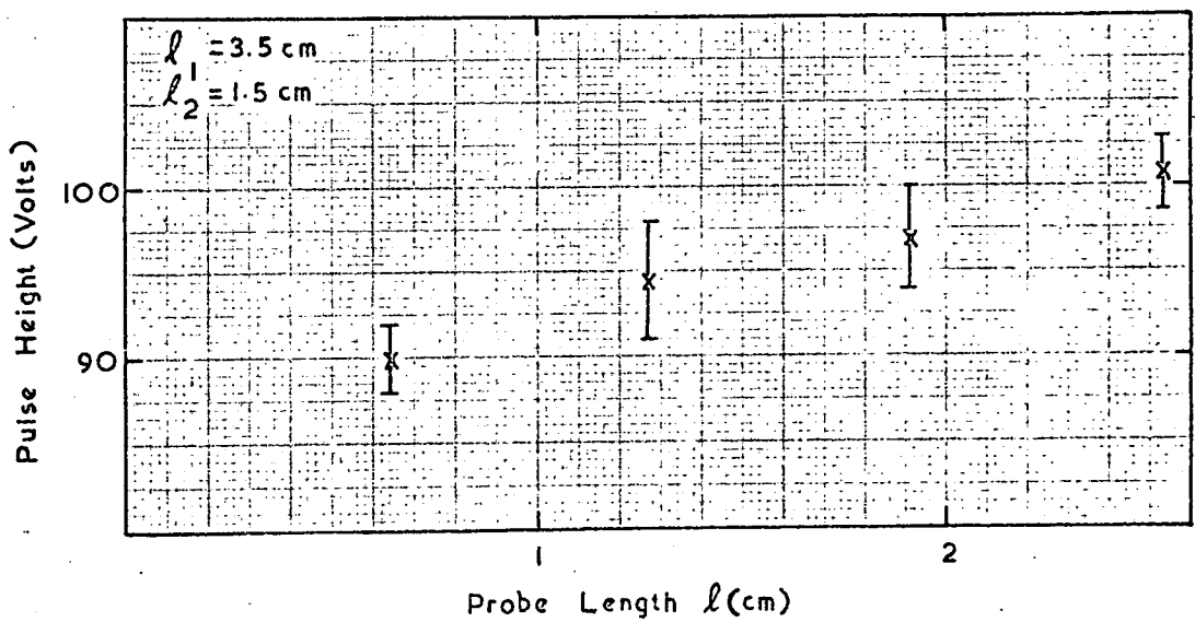
Figure 4.4(b) The Variation of Pulse Height with Probe Length.
