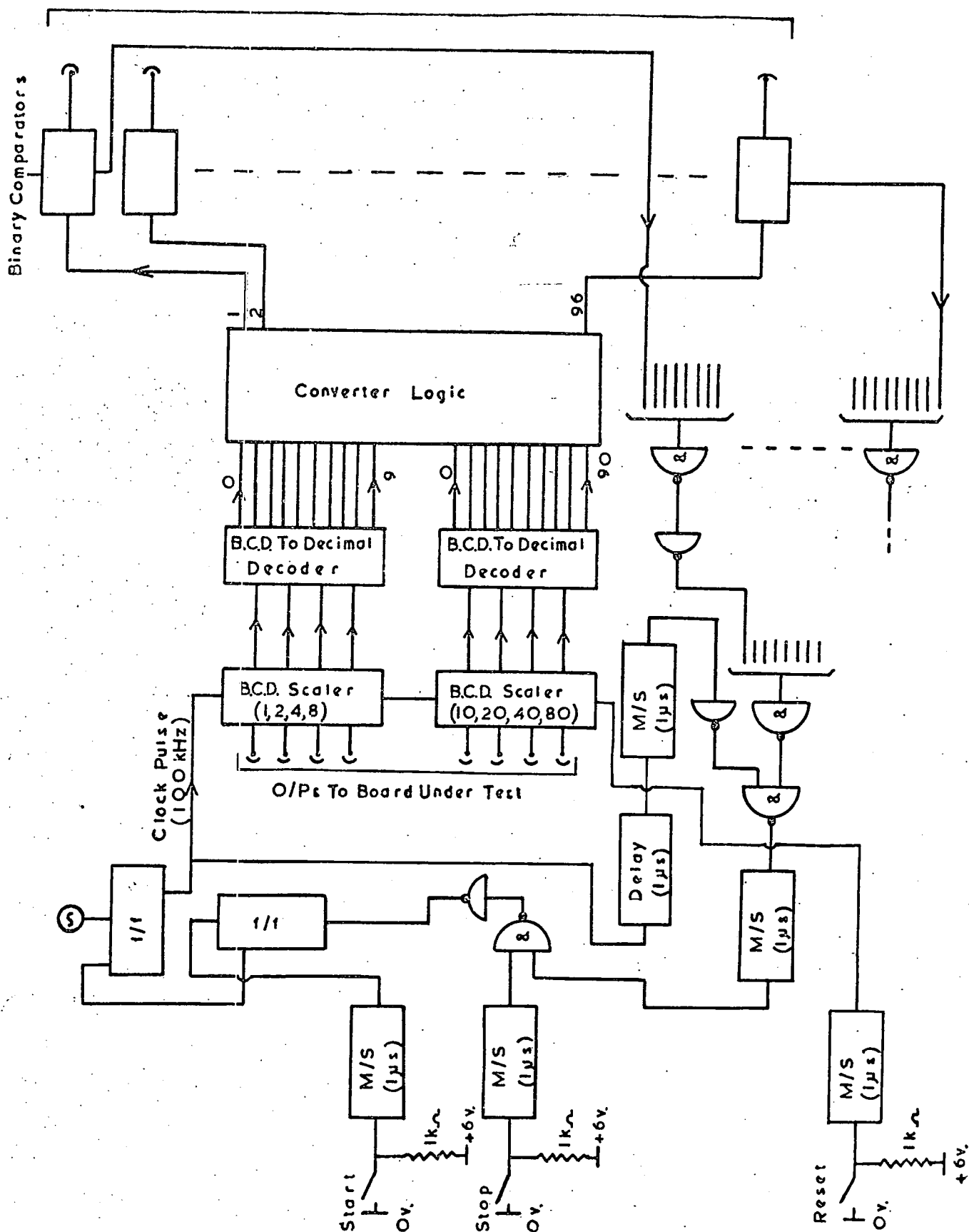
Figure 6.11 The Circuit for the Gating Logic Board Tester.
