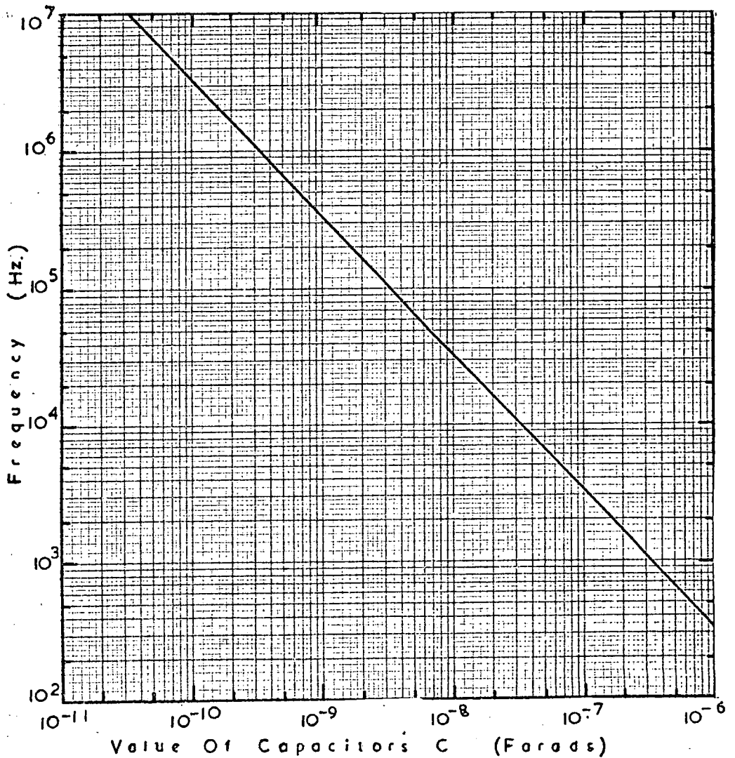
Figure A.4(b) The Variation of Multivibrator Frequency with Capacitors, C.
