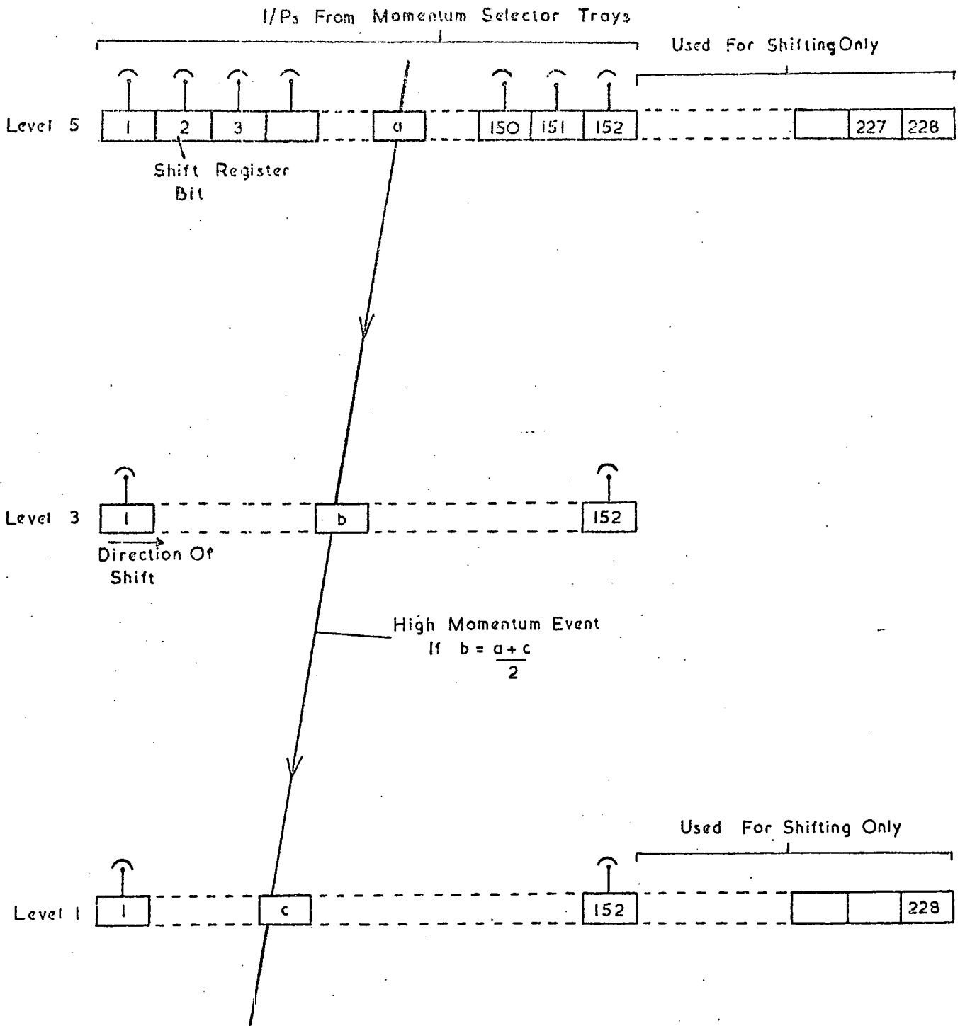
Figure 5.2 The Principle of Operation of the Momentum Selector.
