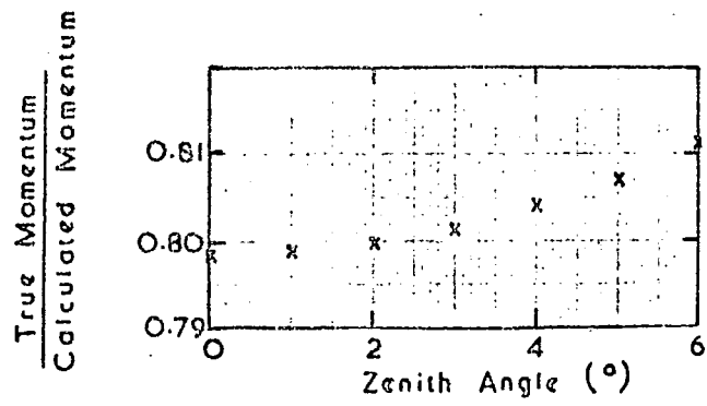
Figure 7.6 The Variation in the Ratio of True Momentum to Calculated Momentum with Zenith Angle.
