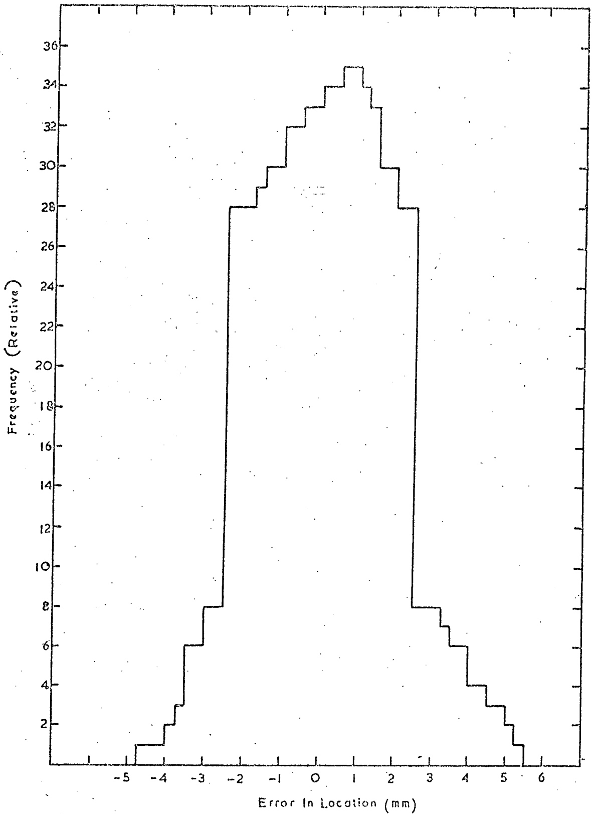
Figure 5.9 Histogram of the Error in Location for a Momentum Selector Tube Spacing.
