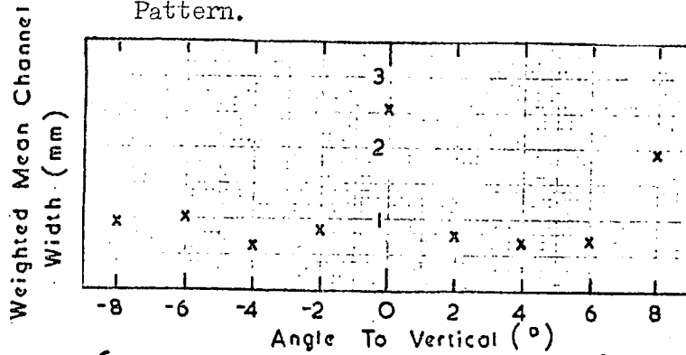
Figure 6.3(a) Graph of the Variation of Weighted Mean Channel Width With Angle for the Flash Tube Pattern of Figure 6.3(b).
