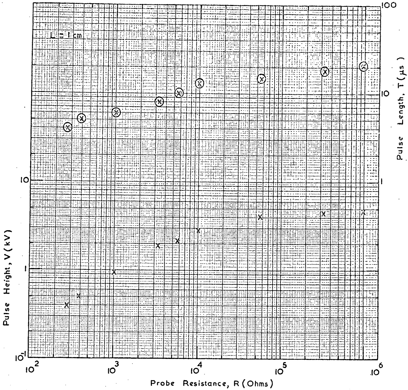
Figure 4.11 The Variation of Pulse Height and Length with Probe Resistance for an Applied Negative High Voltage Pulse.
