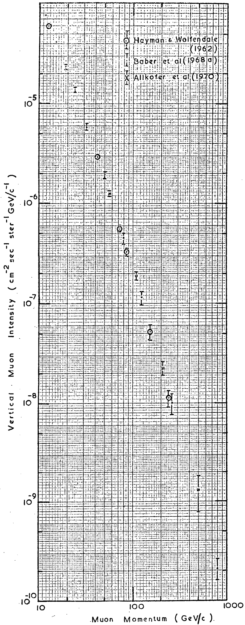
Figure 1.1 The Vertical Muon Differential Momentum Spectrum.
