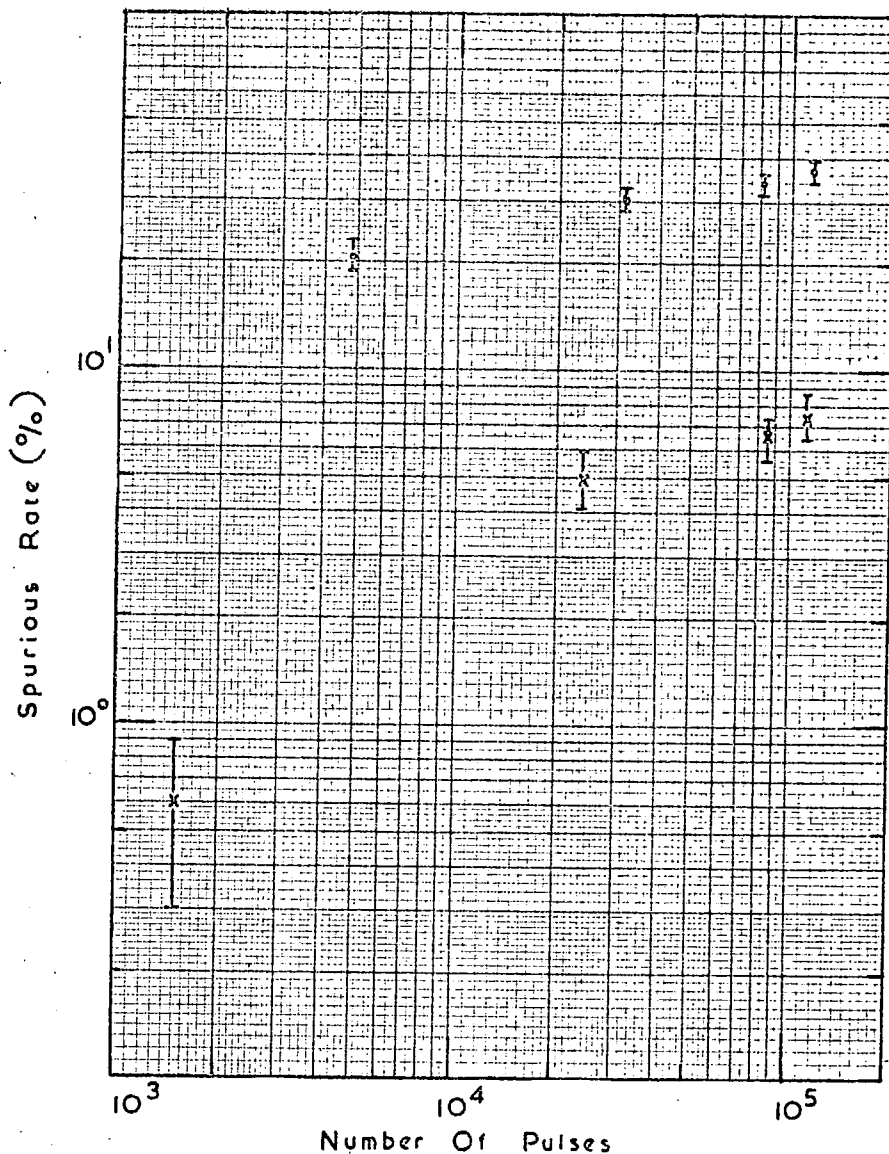
Figure B.4 Graphs of the Spurious Rate against Number of Pulses for Different Exponential Pulse Lengths.
