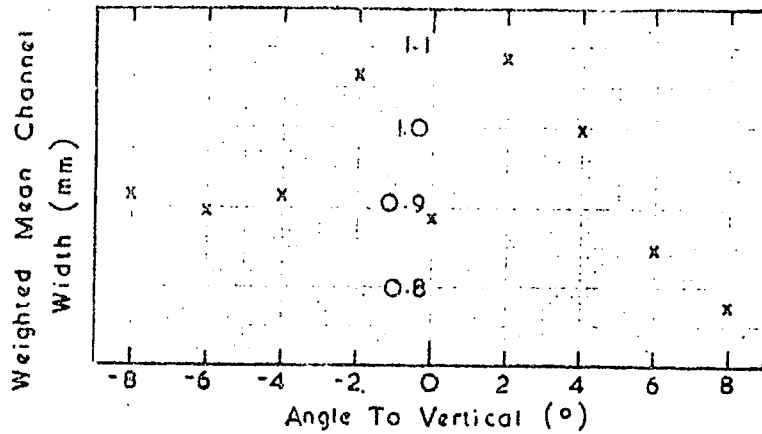
Figure 6.2 Graph of the Variation of Weighted Mean Channel Width with Angle for the Measuring Tray Pattern.
