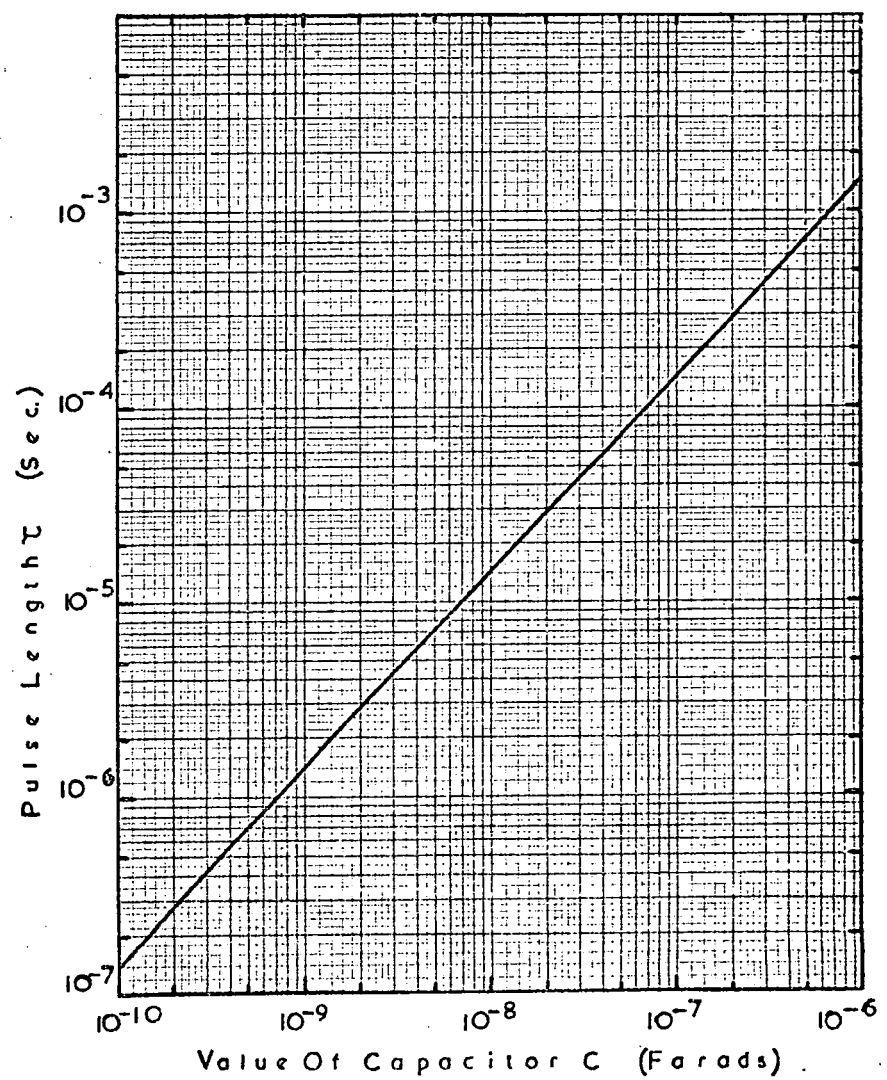
Figure A.2(b) The Variation of Pulse Length, \tau , with Capacitor, C.
