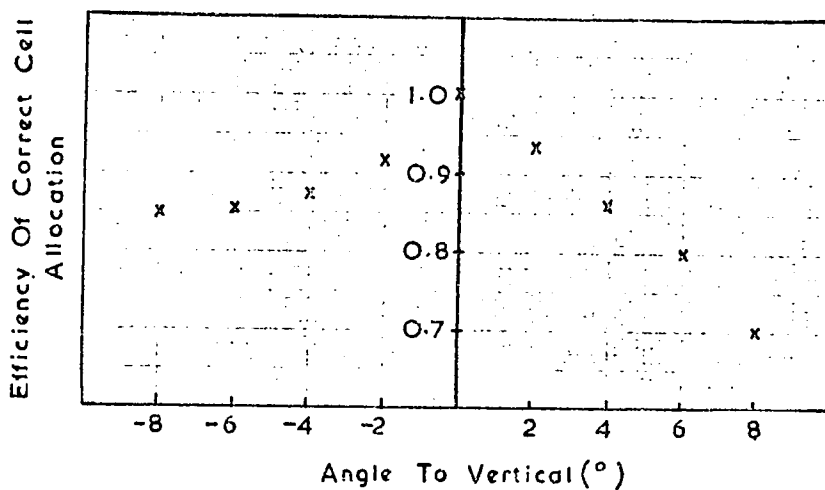
Figure 5.8 The Variation of the Efficiency of Correct Cell Allocation with Incoming Angle.
