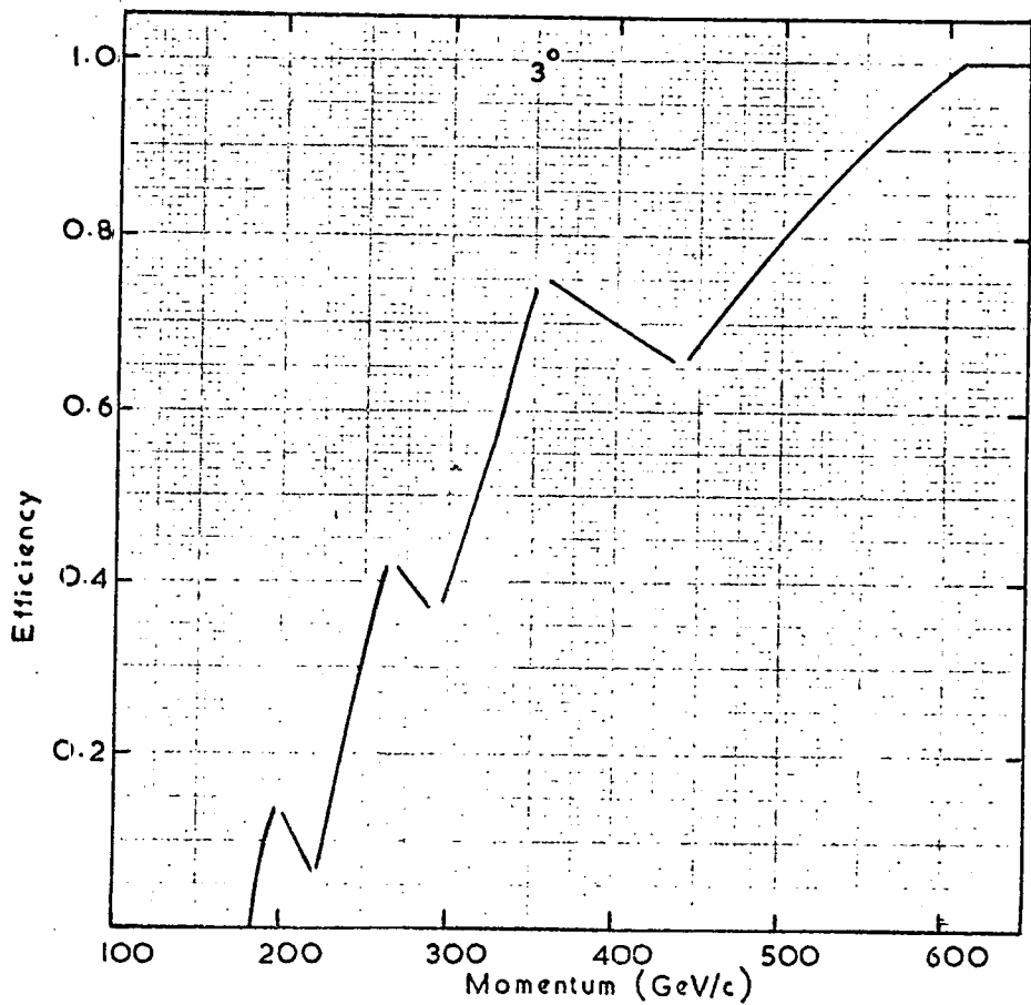
Figure 7.2(b) The Variation in the Efficiency of the Momentum Selector, for Particles Incident at 3^\circ , with Momentum.
