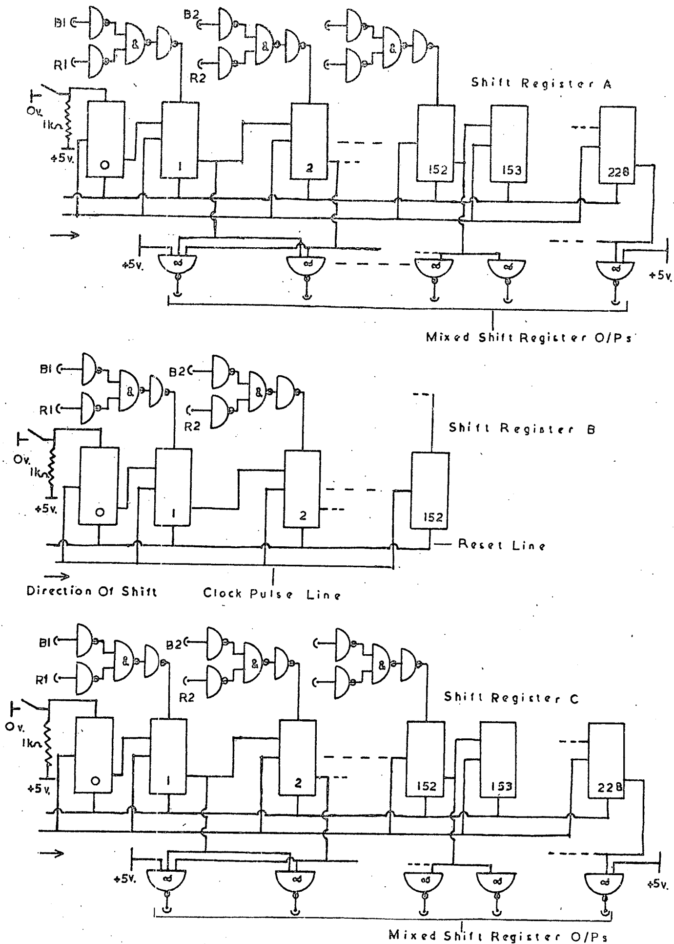
Figure 5.17. The Circuit for the Momentum Selector Shift Registers.
