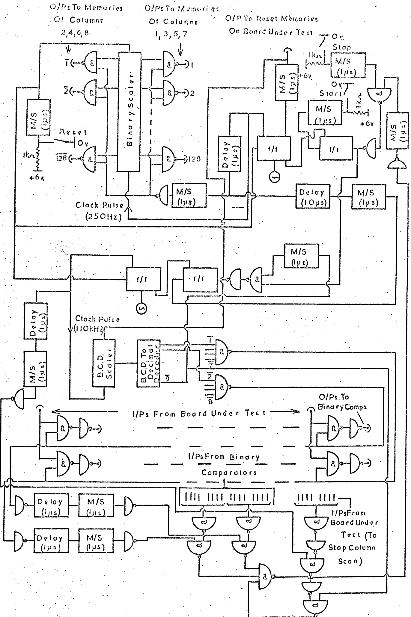
Figure 6.10 The Circuit for the Special Memory Board Tester.
