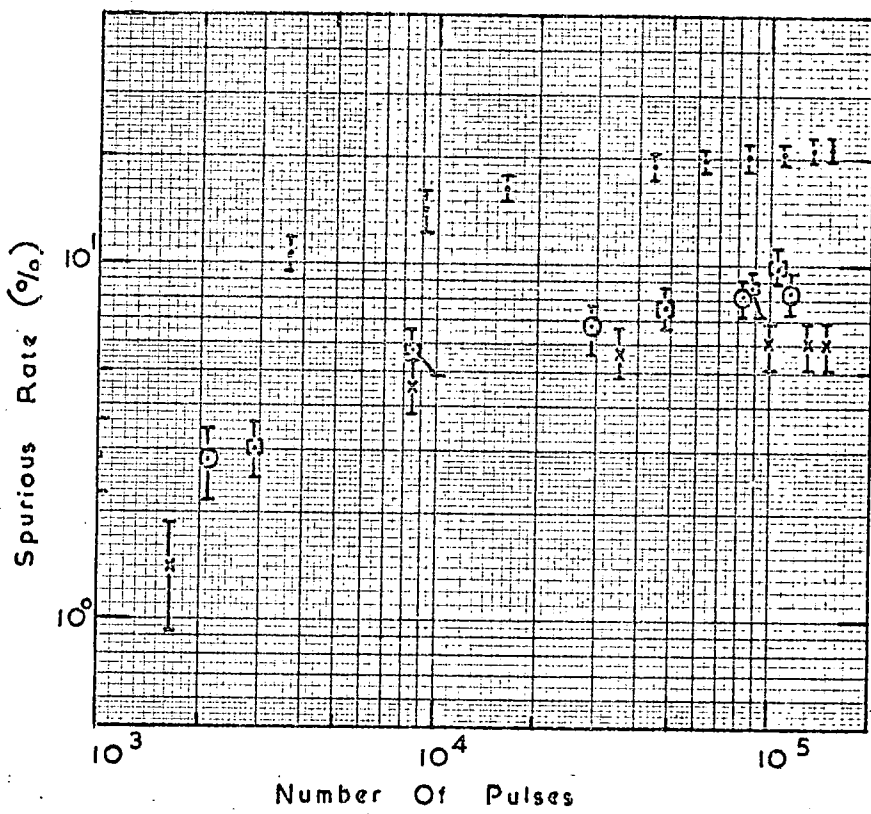
Figure B.3 Graphs of the Spurious Rate against Number of Pulses for Various Electrode Sizes.
