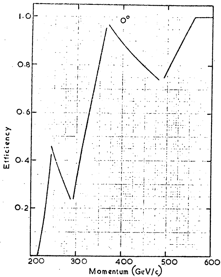
Figure 7.2(a) The Variation in the Efficiency of the Momentum Selector, for Particles Incident at 0^\circ , with Momentum.
