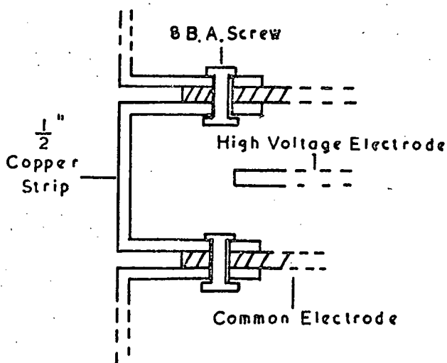
Figure 5.5 The Method of Interconnecting the Electrodes of a Flash Tube Tray.
