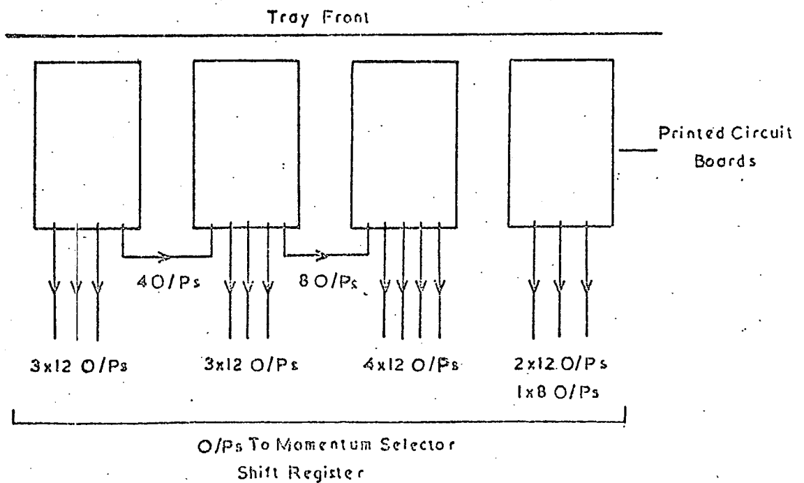
Figure 5.15. The Arrangement of the Cell Allocation Printed Circuit Boards in a Tray.
