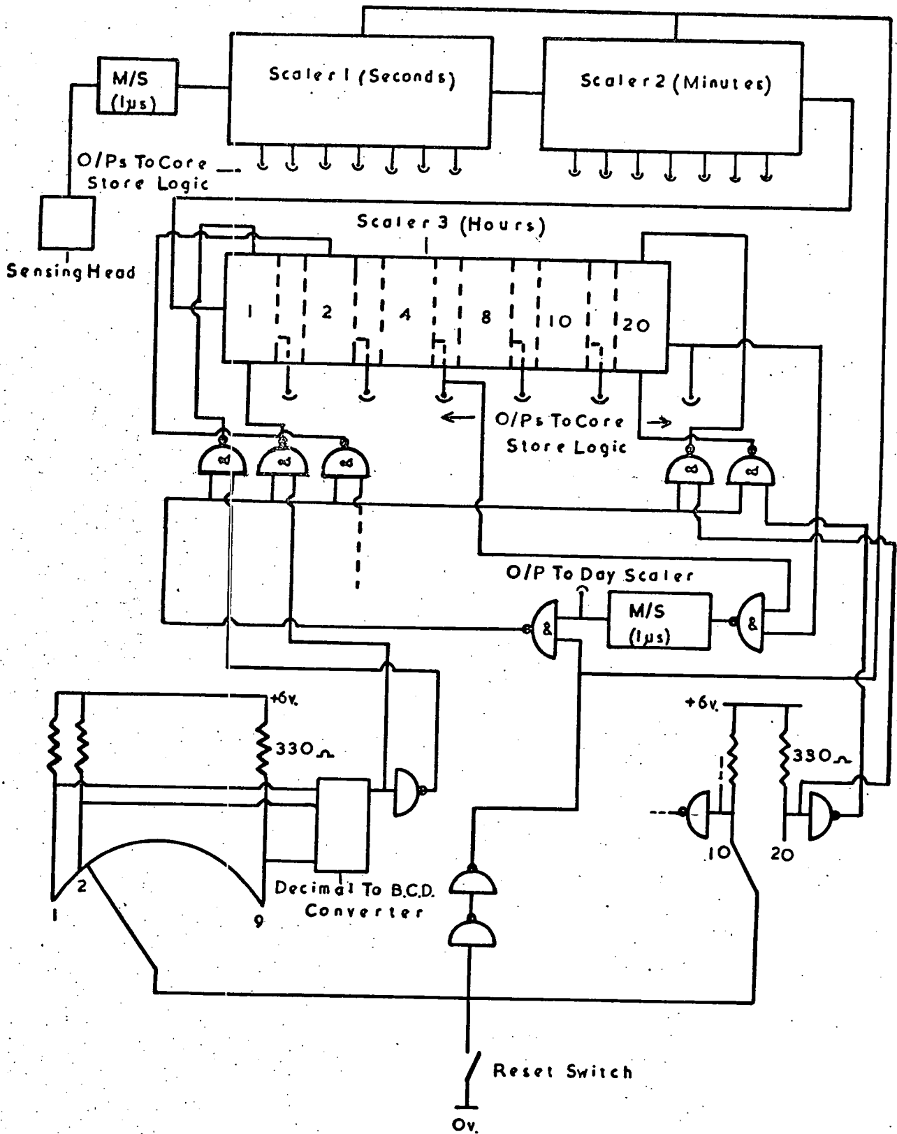
Figure 6.18 The Circuit for Digitising the Time of the Event.
