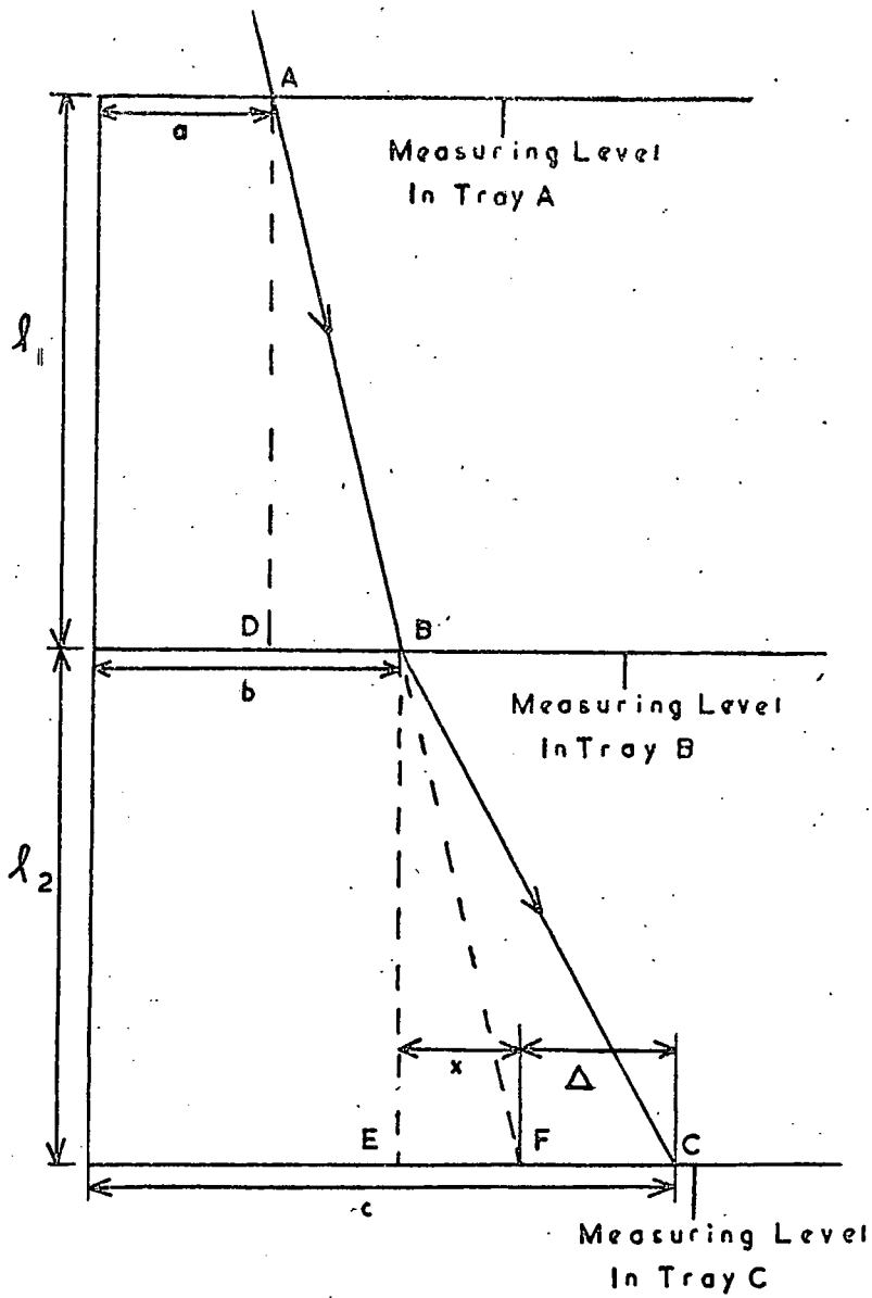
Figure 7.1 The Co-ordinates and Deflection of a Particle Measured in the Momentum Selector Trays.
