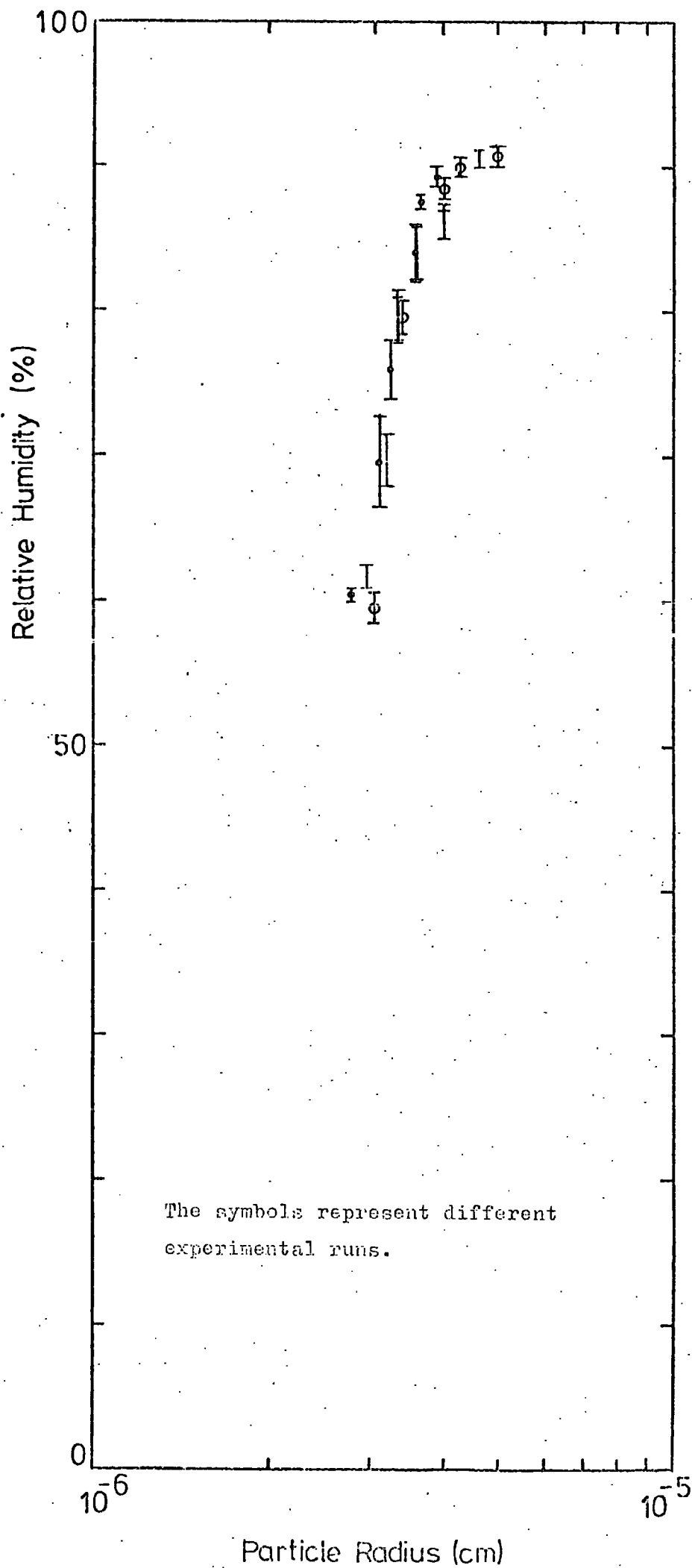
Figure 4.4 Experimental growth of ammonium sulphate.
