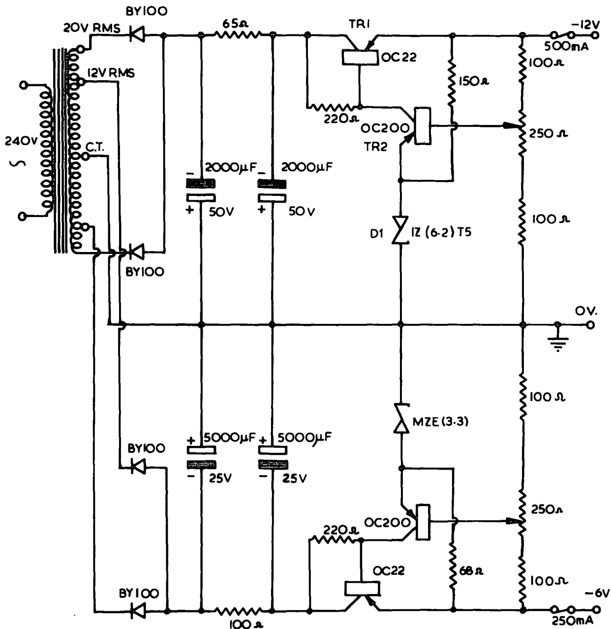
Fig. 3.6. Regulated Power Supply for -12V & -6V.
