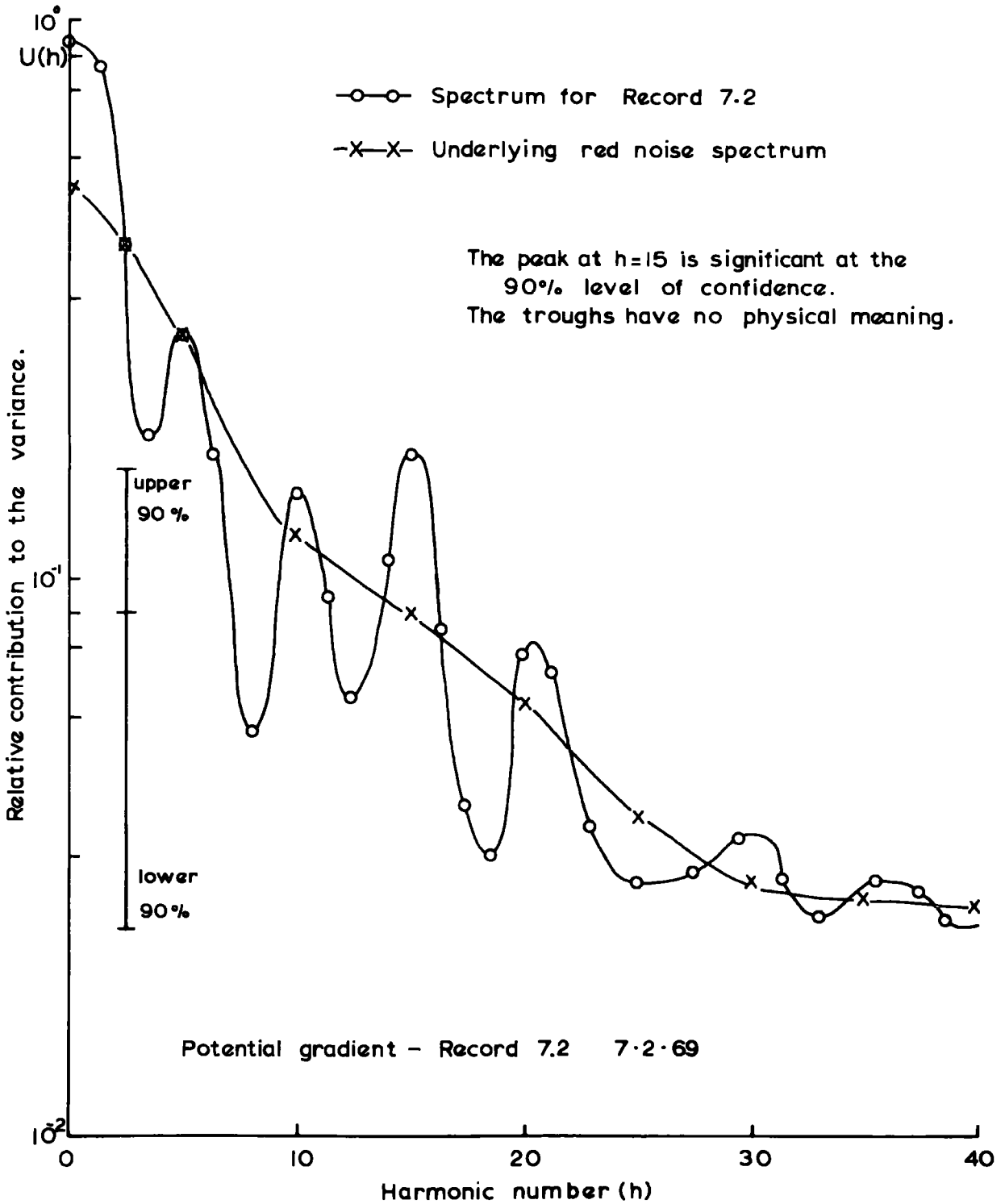
Fig. 5.7. Significance levels for peaks in the variance spectrum.
