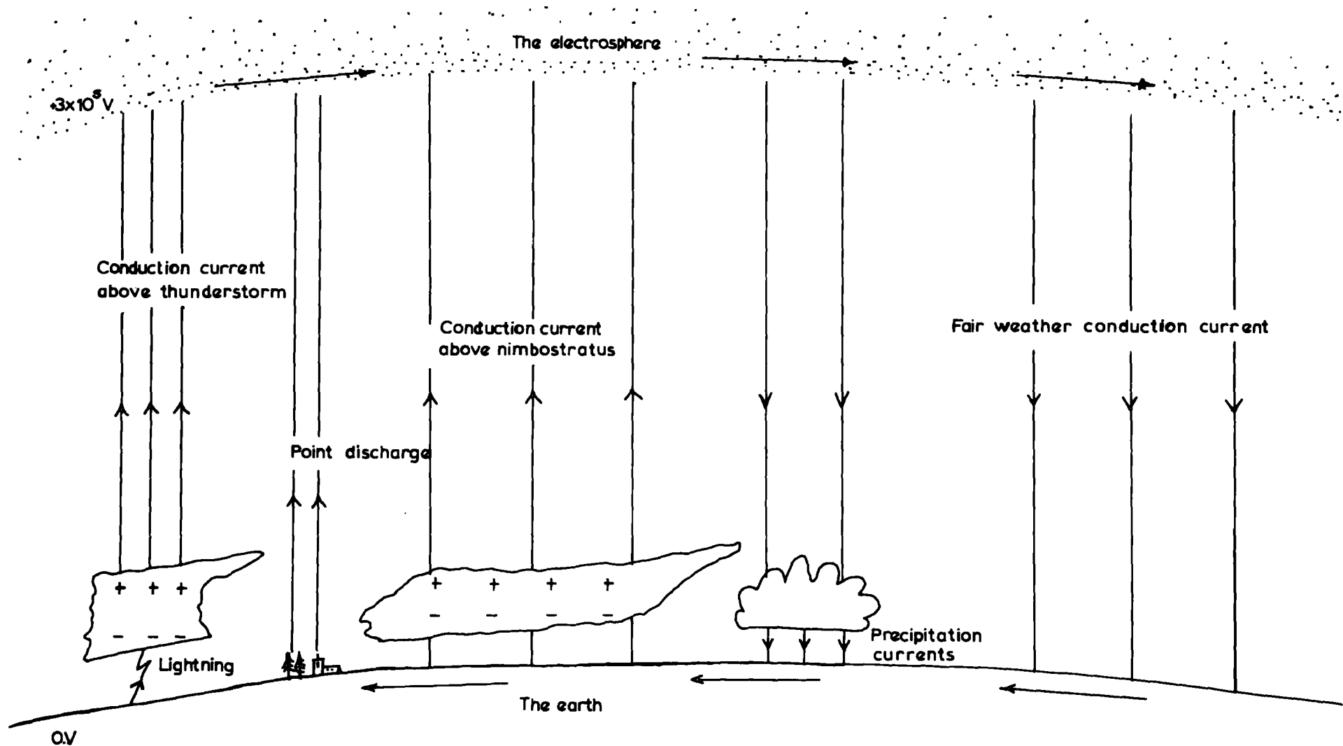
Fig.1.1. The electrosphere - earth currents.
