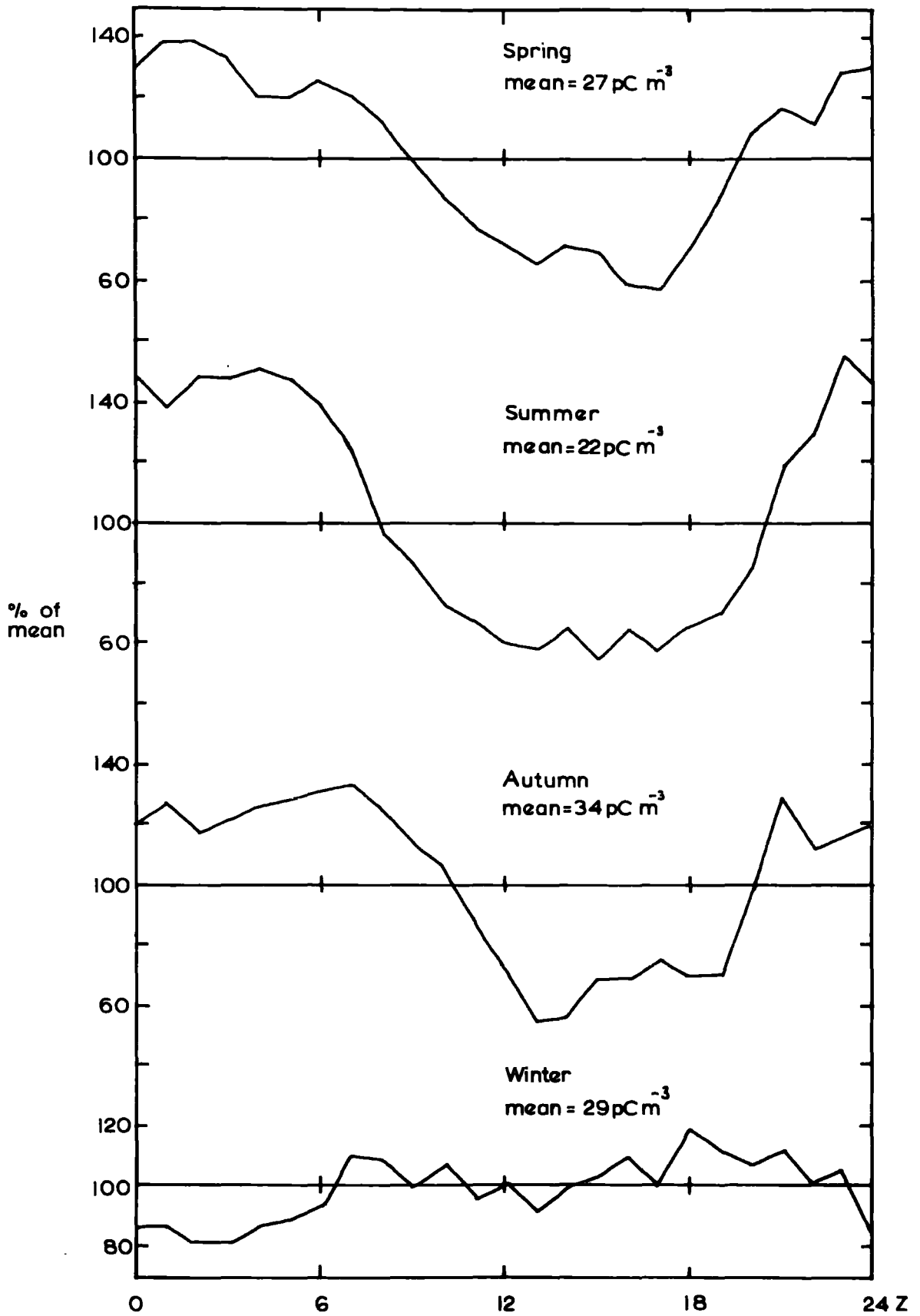
Fig. 8.7. Seasonal variation in space charge density. July 1967- July 1969
