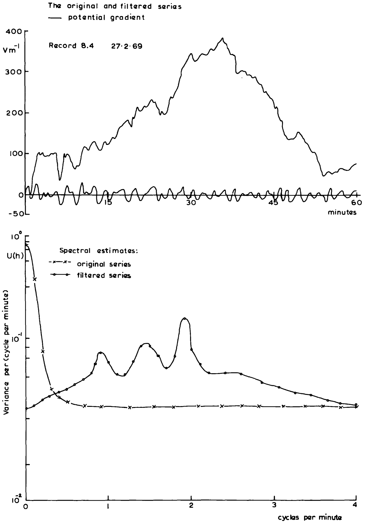
Fig. 5.6. Removal of trends from time series.
