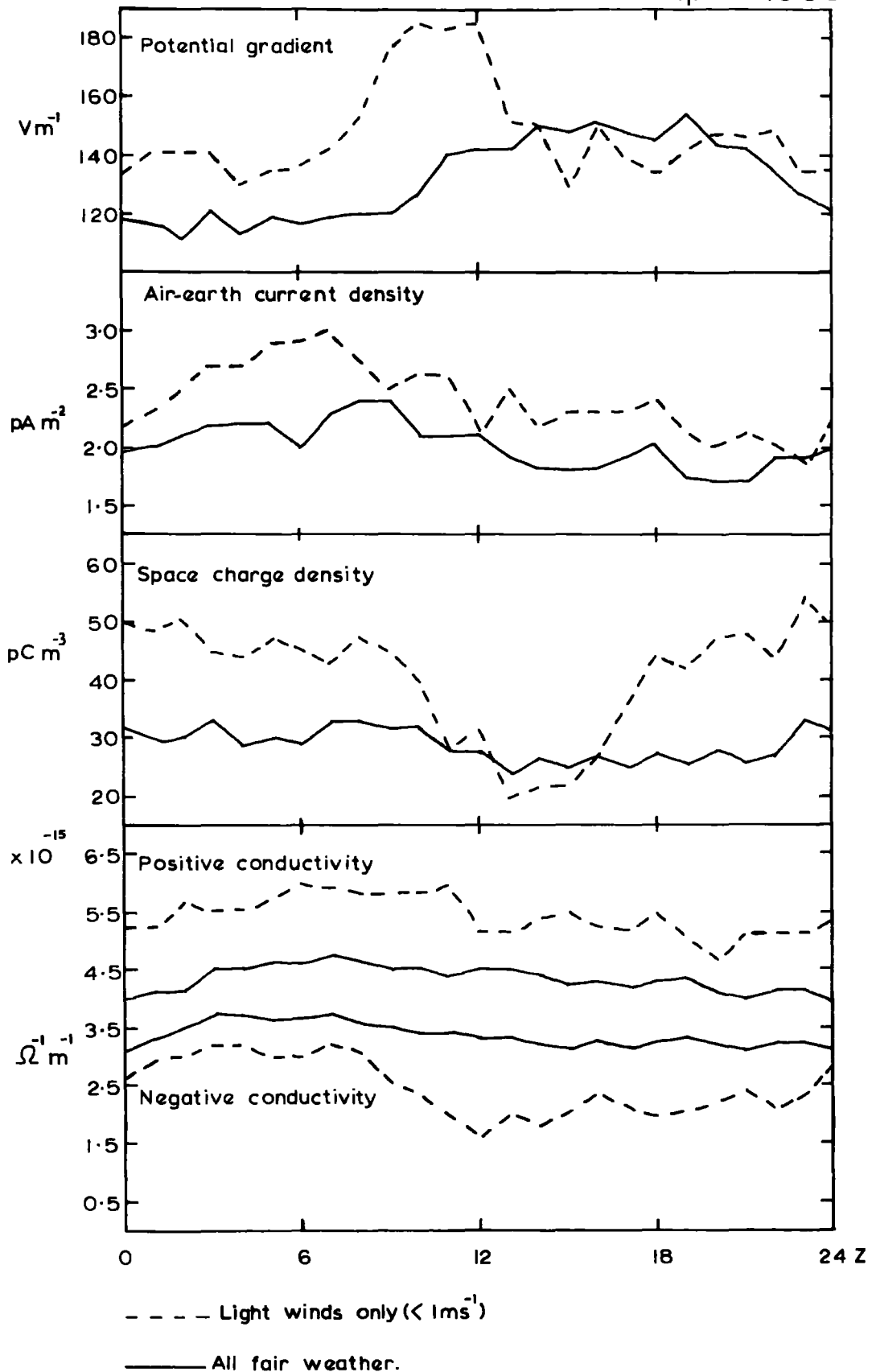
Fig. 8.9. The effect of light winds on the diurnal variations.
