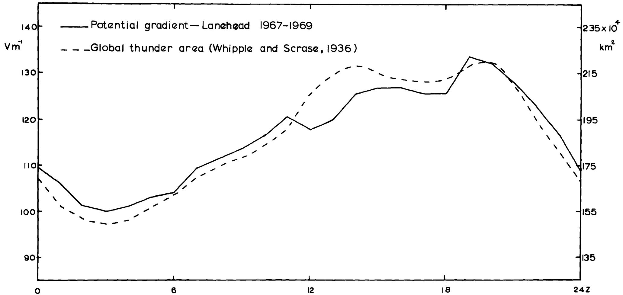
Fig. 8.3. Diurnal variations of potential gradient and World-wide thunderstorm activity.
