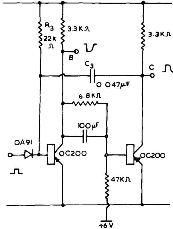
Monostable Multivibrator
