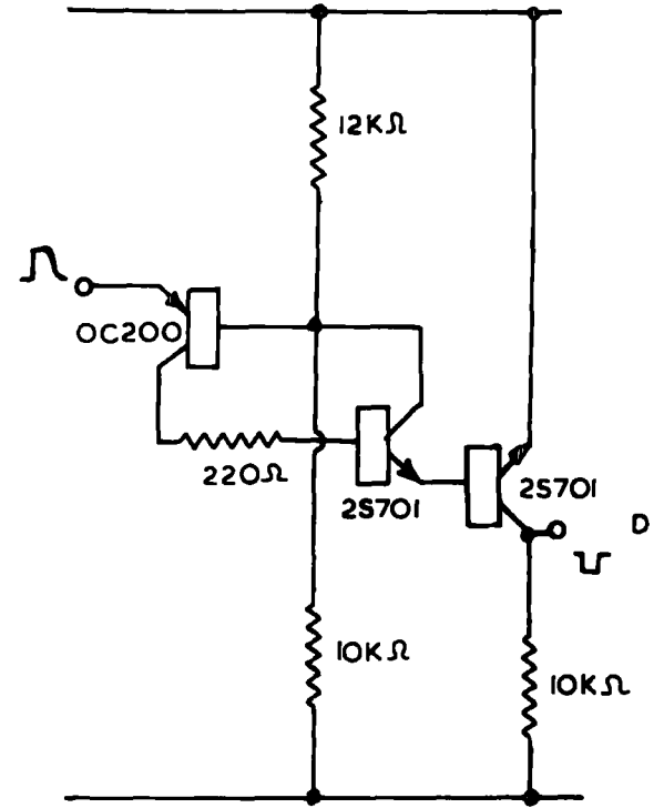
Pulse Shaper
