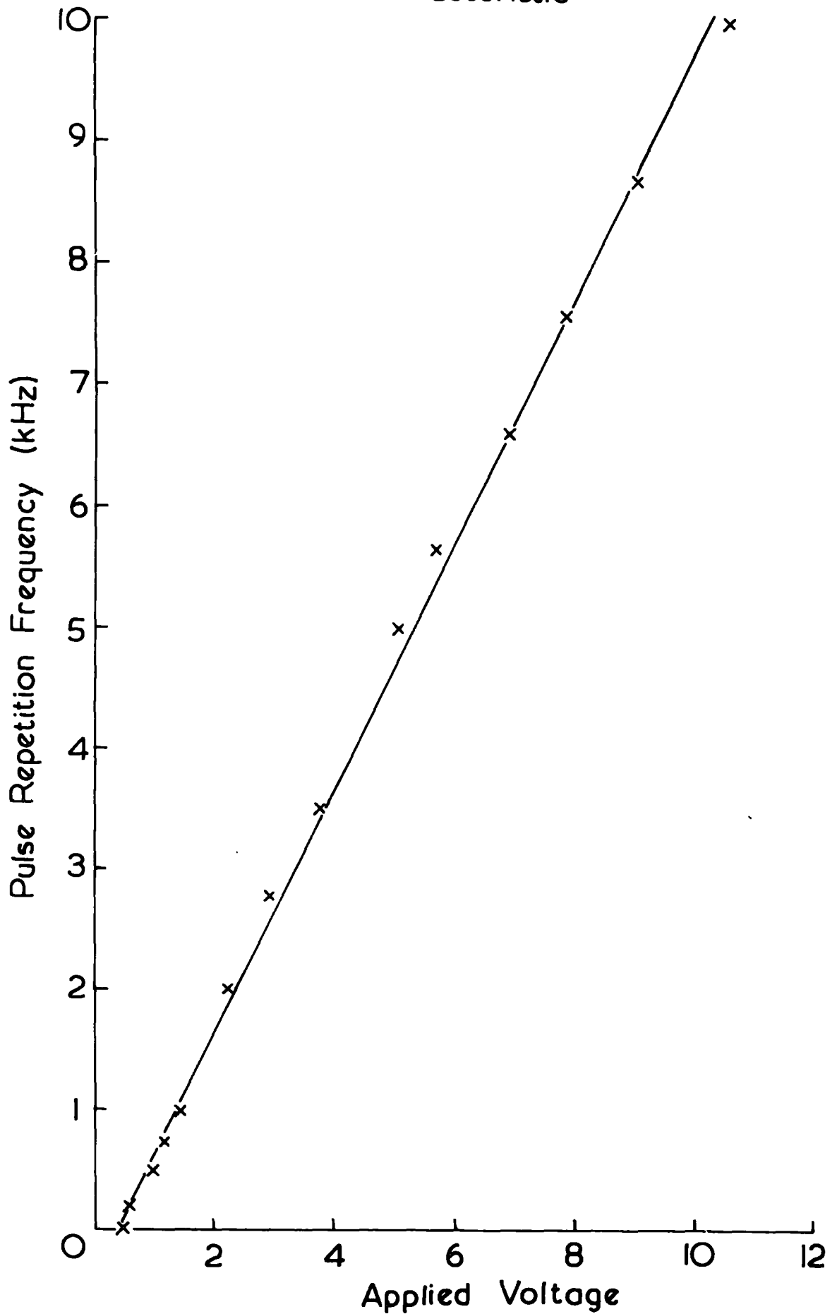
Fig. 3.9. Voltage-to-Frequency Conversion Characteristic
