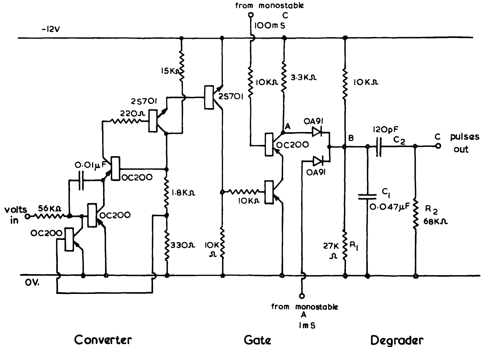
Fig.3.8. The Voltage to Frequency Converter.
