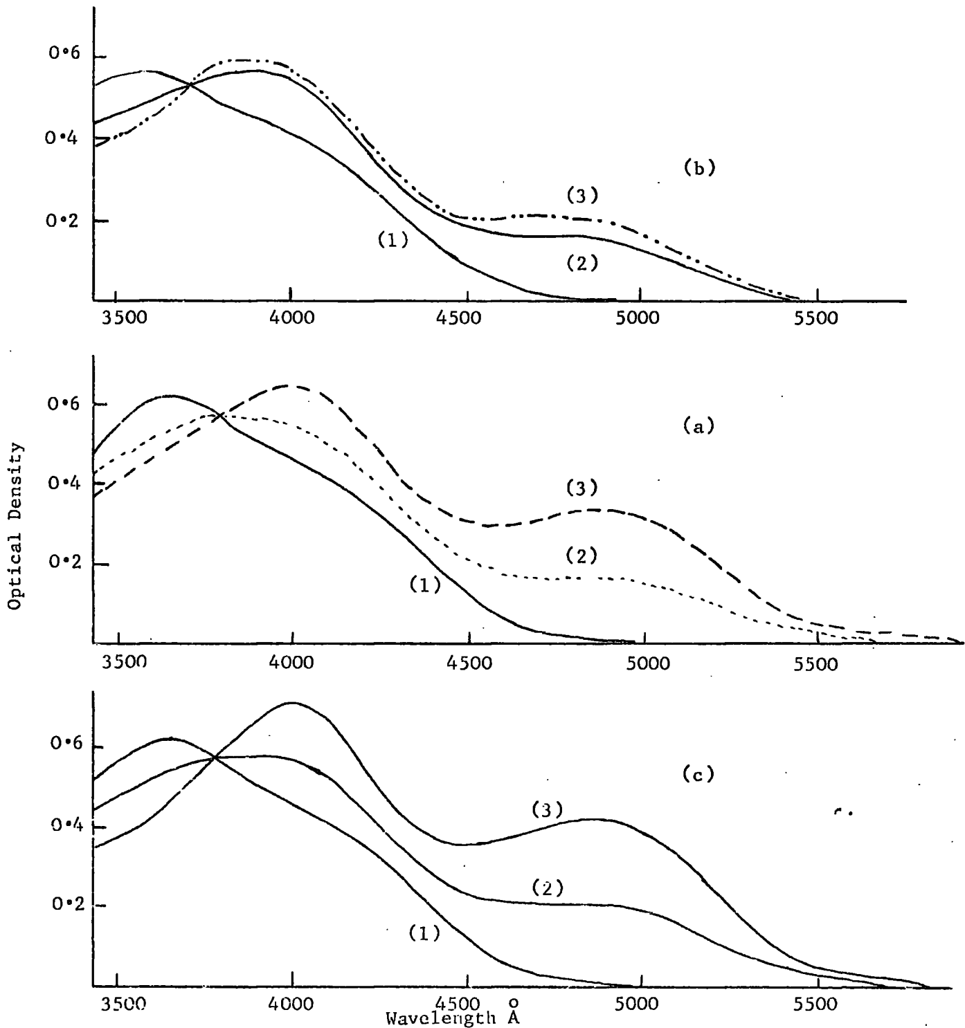
Fig.4. Visible absorption spectra of picric acid ( 4 \times 10^{-5} \text{ M} ) in a - 4:1 (v/v) water-DMSO with [\text{Na}_2\text{SO}_3] \text{M} : 1, 0.00; 2, 0.14; 3, calculated spectrum for complete conversion to complex A, b - 3:2 (v/v) water-DMSO with [\text{Na}_2\text{SO}_3] \text{M} : 1, 0.00; 2, 0.03; 3, 0.11, c - 1:1 (v/v) water-DMSO with [\text{Na}_2\text{SO}_3] \text{M} 1, 0.00; 2, 0.02; 3, 0.05.
