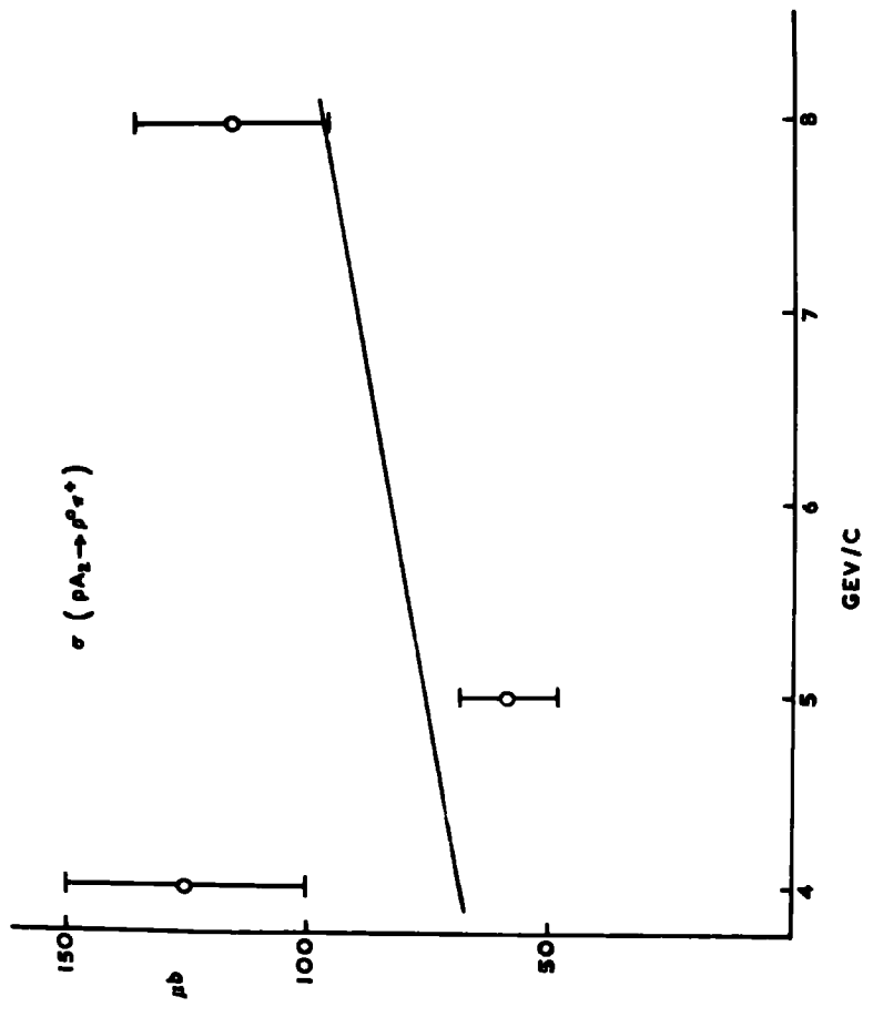
FIG. 5B \sigma(\rho A_2 \rightarrow \rho^0 \sigma^+) vs. MOMENTUM OF INCIDENT \sigma^+
