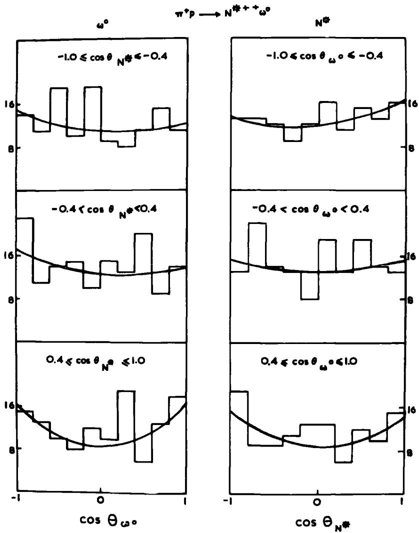
FIG. 41 DECAY ANGULAR CORRELATIONS
