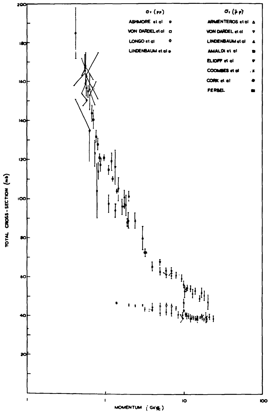
FIG. 1 Total \bar{p}p and pp cross-sections
