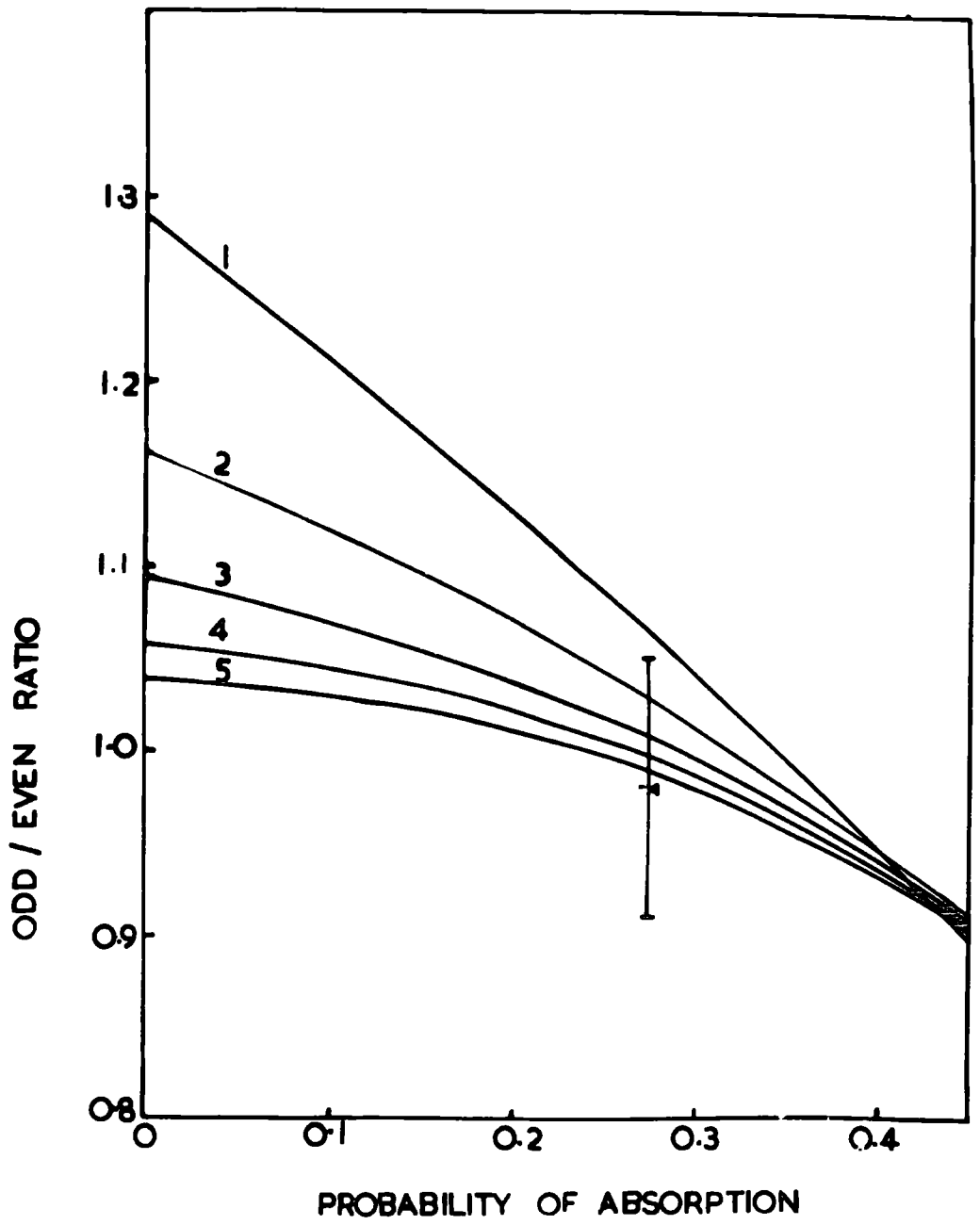
FIG 8 The calculated variation of odd even ratio due to absorption and charge exchange of secondary mesons
