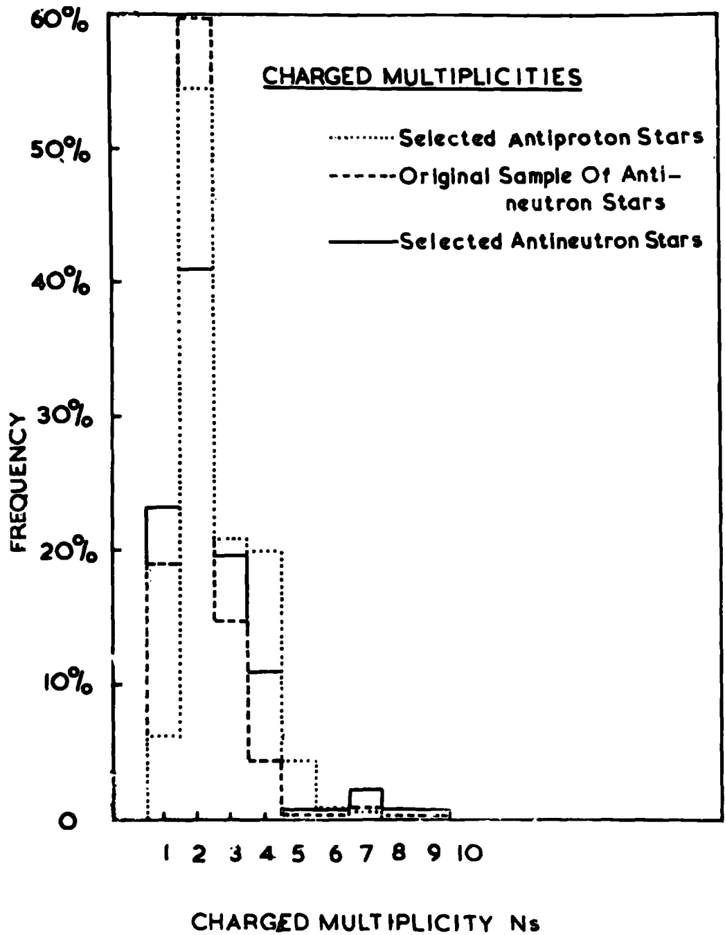
FIG.24 The comparison of charged multiplicities
