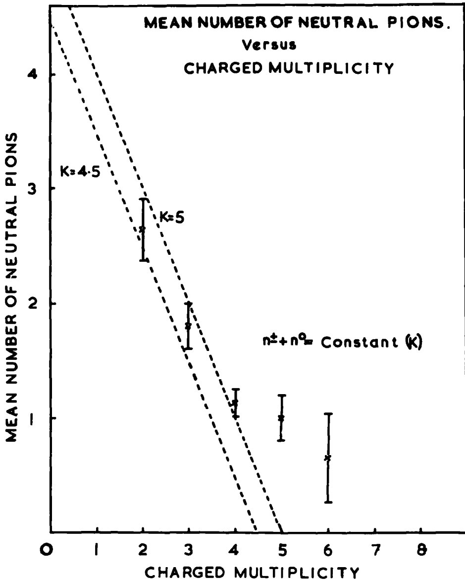
FIG. 5 Mean number of neutral pions accompanying particular charged multiplicities
