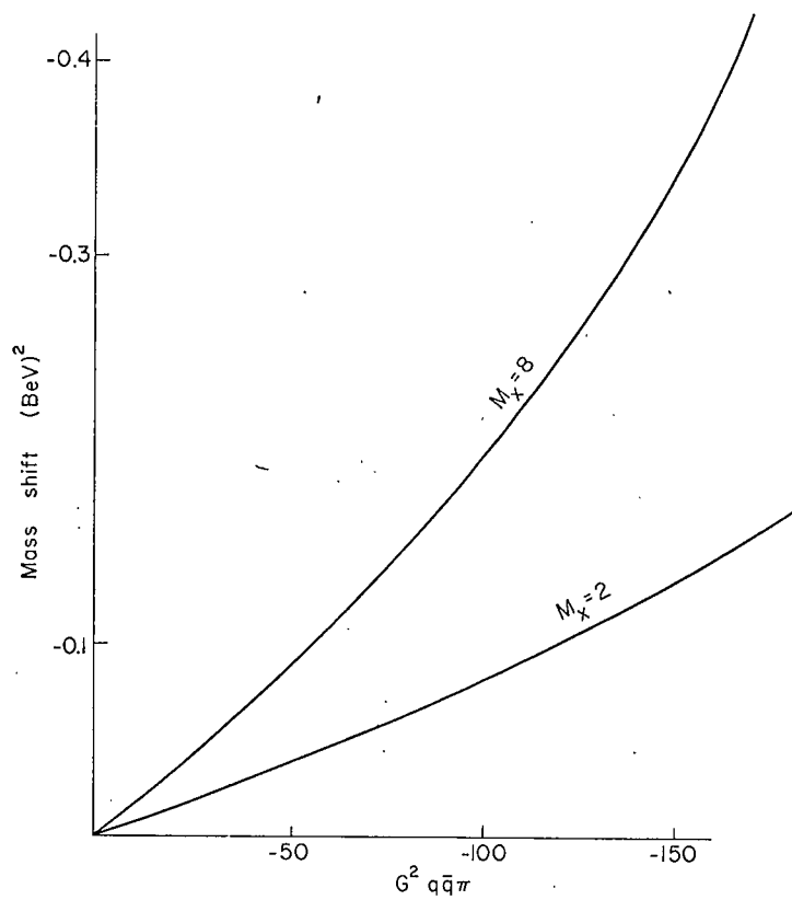
FIG. 2. The variation of the shift of the \rho mass with G_{q\bar{q}\pi}^2
