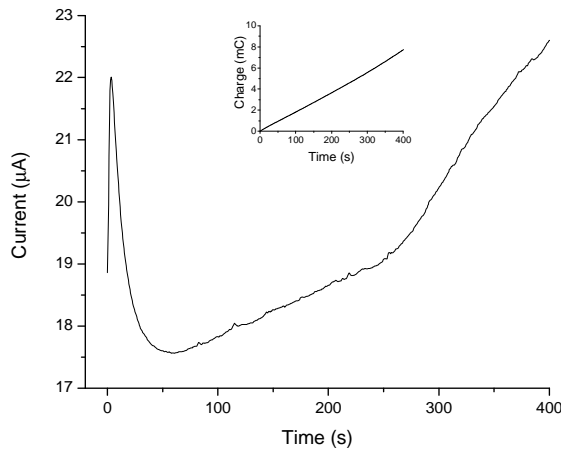
Figure 3: Current transient recorded during the electropolymerization of a mixture of 0.01 M EDOT, 0.0125 M PSS and 12.5 mg/ml FluidMAG-PS in the pores of a PC membrane having an adsorbed layer of avidin on the pore walls. The inset shows the charge vs. time during polymerization.
