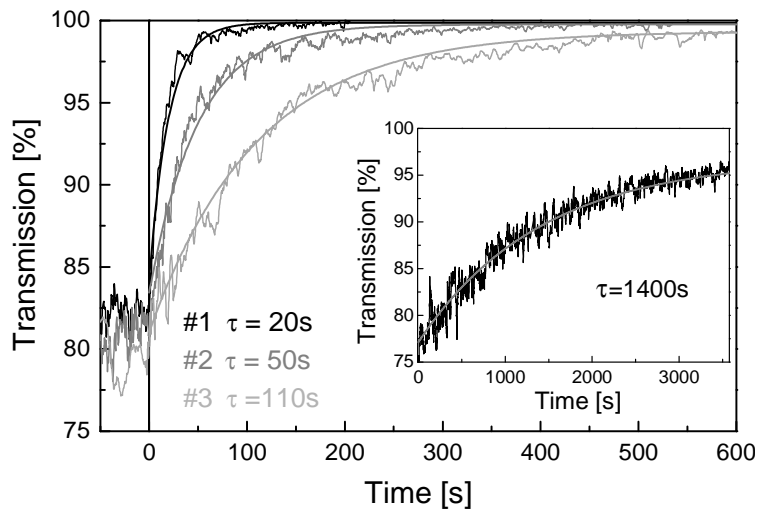
Figure 7: Temporal dependence of the light transmission in aqueous PEDOT:PSS microrod suspensions in static magnetic fields used to collect the rods from the suspensions. The different curves (#1, #2 and #3) correspond to different strength of the magnetic field as summarized in Table 1. Insertion of the magnet corresponds to t=0 s. The results of fitting with exponential decay according to the formula T=1-c \cdot \exp(-t/\tau) are also indicated by dashed lines for each curve in the graph together with the corresponding values of the relaxation time, \tau . The inset shows time dependence of the light transmission measured without magnetic field (curve #4).
