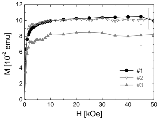
Figure 6: Magnetization curves of the FluidMAG-PS nanoparticles (curve#1) and the PEDOT:PSS microrod samples (two independent batches: curve #2 and #3) normalized to 1 mg quantity of. (The error bars for the microrod samples are mostly related to the uncertainty of the magnetite content determination. The reproducibility of the magnetization measurement introduces negligible error.)
