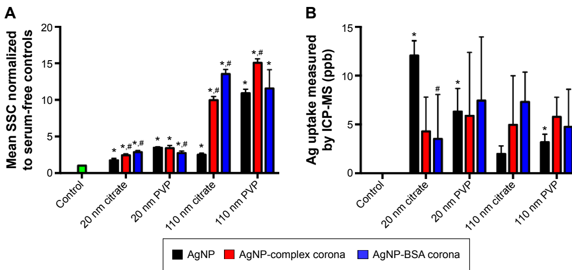
Figure 5 Measurement of AgNP uptake by assessment of changes in SSC via flow cytometry and ICP-MS. Notes: Macrophages were exposed to AgNPs, AgNPs with a complex PC, or AgNPs with a BSA PC at a concentration of 25 µg/mL for 2 hours, and uptake was determined by (A) assessment of changes in SSC shift and (B) ICP-MS analysis of silver content. SSC values of cells exposed to AgNPs were normalized to serum-free media control cells to produce a fold change. Values are expressed as mean ± SEM (n=4–7 per group). *Significant difference from unexposed control cells (P<0.05). #Significant difference compared to AgNP without a PC (P<0.05). Abbreviations: NP, nanoparticle; SSC, side scatter; ICP-MS, inductively coupled plasma-mass spectrometry; PC, protein corona; BSA, bovine serum albumin; SEM, standard error of mean; PVP, polyvinylpyrrolidone.
