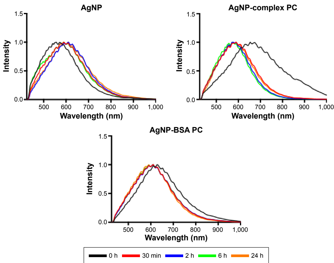
Figure 4 Time course of macrophage internalized in 110 nm PVP-suspended AgNPs. Notes: Macrophages were exposed to AgNPs, AgNPs with a complex PC, or AgNPs with a BSA PC at a concentration of 25 µg/mL for 30 minutes. Following exposure, AgNPs were removed, and cells were washed and placed in media with serum. Spectra of internalized 110 nm AgNPs were assessed at 30 minutes, 2 hours, 6 hours, and 24 hours postexposure. Abbreviations: PVP, polyvinylpyrrolidone; NPs, nanoparticles; PC, protein corona; BSA, bovine serum albumin; h, hours; min, minutes.
