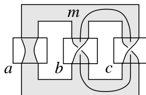
Figure 18: The pretzel knot p(a, b, c) for a = 0, b = 1, c = 1
