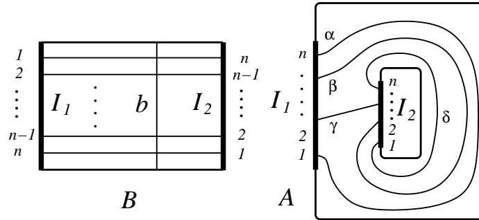
Figure 3: The arcs \omega \cap B \subset B and \omega \cap A \subset A
