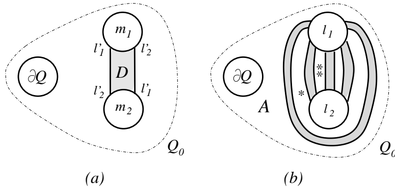
Figure 10: The possible graphs G_{Q_0}
