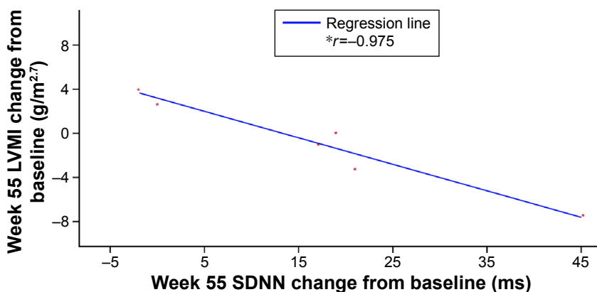
Figure 3 Correlation between change from baseline to week 55 in SDNN and LVMI in patients with baseline SDNN < 100 ms. Notes: * r = Pearson correlation coefficient. SDNN represents the standard deviation of all filtered RR intervals for the length of the analysis. Abbreviation: LVMI, left ventricular mass index.
