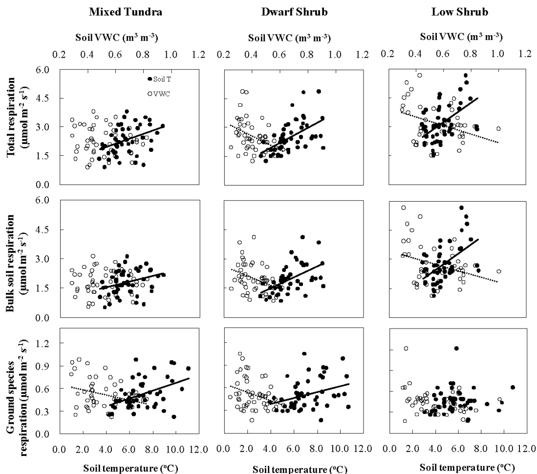
FIGURE 5. Relationship between respiration rates and soil temperature ( ^{\circ}\text{C} ) at 5 cm depth (filled circles) and soil moisture ( \text{m}^3 \text{m}^{-3} ) at 0–12 cm depth (open circles) at mixed tundra (left column), dwarf shrub (middle column), and low shrub (right column) sites. Black lines indicate significant ( P < 0.05 ) linear regressions of respiration rates to soil temperature. Gray lines indicate the linear significant regressions of respiration rates to soil moisture.
