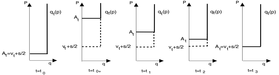
Figure 1: The limit order book and its dynamics. This figure illustrates how the sell side of limit order book evolves over time in response to a sale trade. Before the trade at time t_0 = 0 , the limit order book is full at the ask price A_0 = V_0 + s/2 , which is shown in the first panel from the left. The trade of size x_0 at t = 0 “eats off” the orders on the book with lowest prices and pushes the ask price up to A_{0+} = (F_0 + s/2) + x_0/q , as shown in the second panel. During the following periods, new orders will arrive at the ask price A_t , which fill up the book and lower the ask price until it converges to its new steady state A_t = F_t + \lambda x_0 + s/2 , as shown in the last panel on the right. For clarity, we assume that there are no fundamental shocks.
