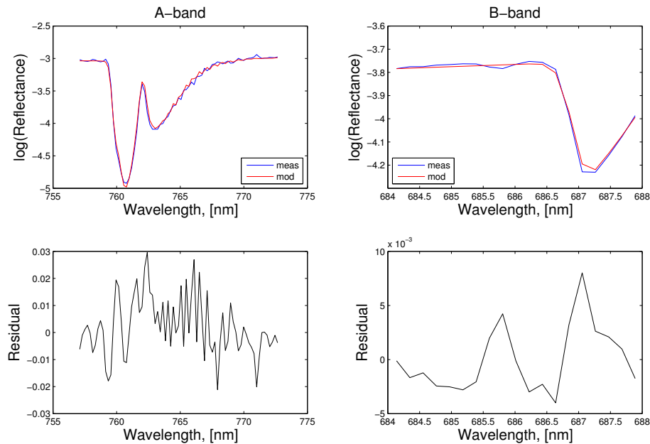
Fig. 8. A fit showing the O 2 A- and B-band spectra simulated by the forward model (red) against the spectra measured by SCIAMACHY (blue), in the upper left and right panels respectively. The log(Reflectance) indicates the natural logarithm of the measured and modeled reflectances. The bottom panels show the corresponding dimensionless residuals \left(\frac{\log R_{\text{mod}} - \log R_{\text{meas}}}{\log R_{\text{meas}}}\right) given here by the difference of the two spectra relative to the measurement.
