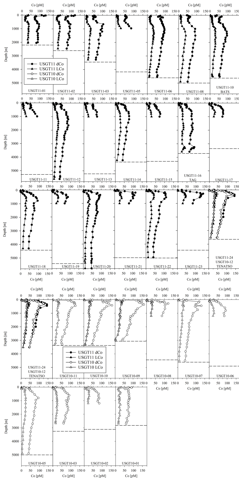
Figure 3. Dissolved profiles of total and labile cobalt for USGT10 and USGT11. Stations of note include USGT11-10 (BATS), USGT11-16 (TAG), USGT10-09 (station closest to the Mauritanian coast), USGT11-1 to USGT11-08 (stations along Line W).
