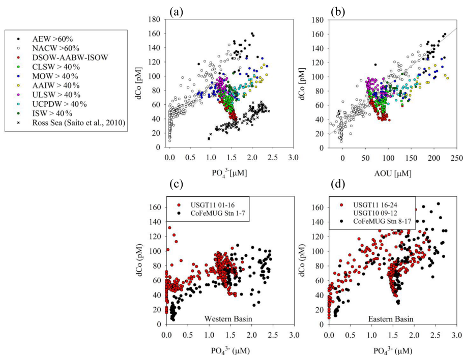
Figure 13. Full depth relationships of total dissolved cobalt, phosphate, and apparent oxygen utilization (AOU). In a comparison with water mass analysis from the GA03 expeditions, clear populations of data by water mass origin were observed in both (a) dCo : P and (b) dCo : AOU space. Data from the Ross Sea is also shown as a potential end member (Saito et al., 2010). dCo : P relationships and the “cobalt curl” deviance from them were observed in the (c) western and (d) eastern basins of the Atlantic, and were similar between the North and South Atlantic (South Atlantic data from Noble et al., 2012).
