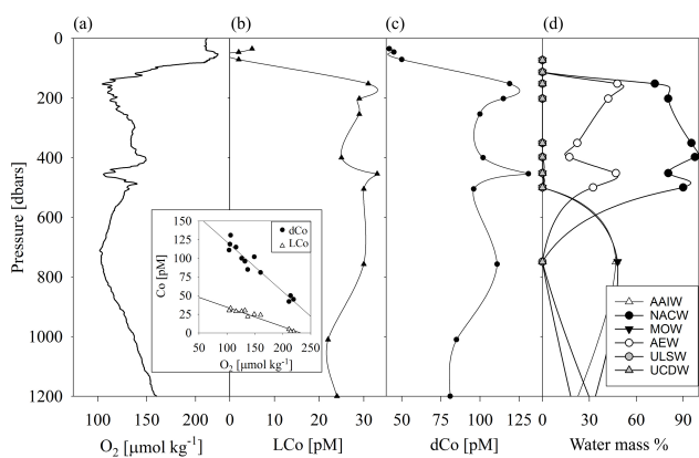
Figure 14. Intermediate depth profile for (a) O_2 , (b) labile cobalt (c) total cobalt and (d) water mass as a percent for USGT10-07. A strong linear correlation with O_2 is observed (inset). A small but distinct maximum is observed between 400 and 600 m and demonstrates the capability of water mass features to influence the cobalt vertical profile at these depths.
