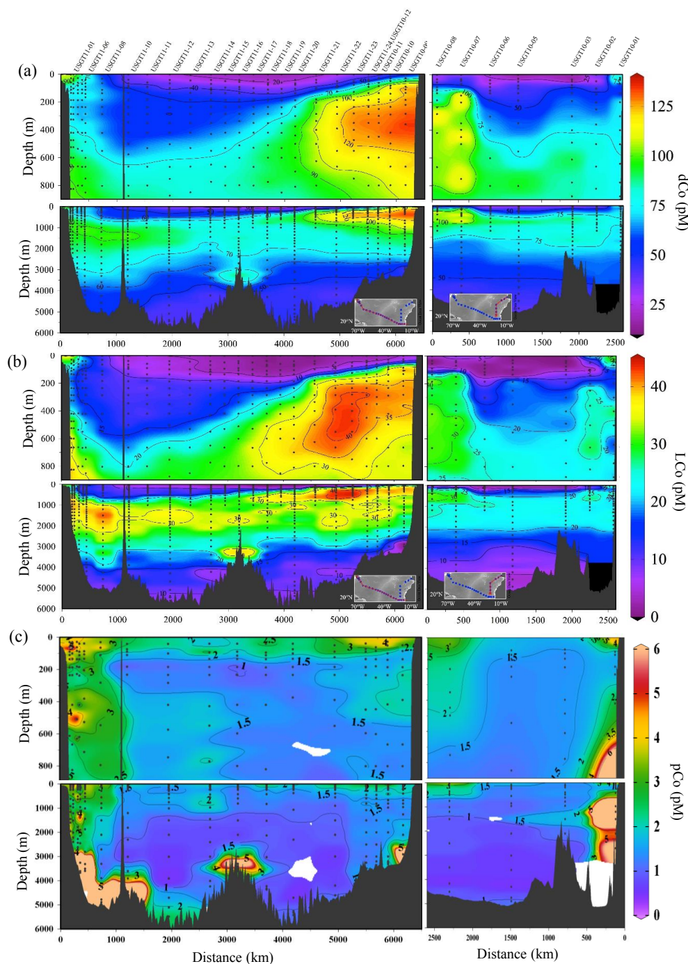
Figure 2. (a) Full depth section of total cobalt, (b) full depth section of labile cobalt, and (c) full depth section of particulate cobalt with the meridional section in the right panels and the zonal section in left panels. These ocean sections were created using Ocean Data View. The dissolved sections were created using “VG” gridding and extrapolated lengths of less than 70% in either y or x direction for any of the section representations.
