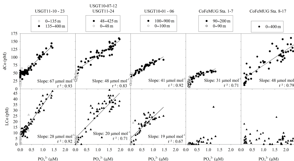
Figure 11. Co : P ecological stoichiometry observed across different regions in the North and South Atlantic. A tighter correlation is observed where labile cobalt becomes detectable and the correlation is observed down to differing depths depending on the strength of the processes that affect cobalt and phosphate biogeochemical cycling. Processes that affect both species similarly in time and space will tend to tighten the correlation and deepen the depth to which it is observed (e.g., USGT10-01–USGT10-06). Where scavenging or reductive dissolution may influence the two species differently, the correlation may be more diffuse or not observed at all (e.g., CoFeMUG Sta. 8–17).
