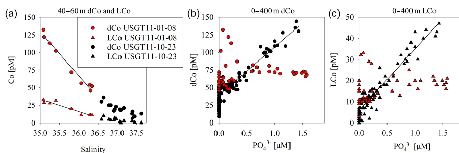
Figure 6. Along Line W, strong relationships between (a) salinity and total cobalt and salinity and labile cobalt were observed in surface waters. Total and labile cobalt show strong correlations with phosphate in the North Atlantic Subtropical Gyre, but this relationship is not observed along Line W (b, c).
