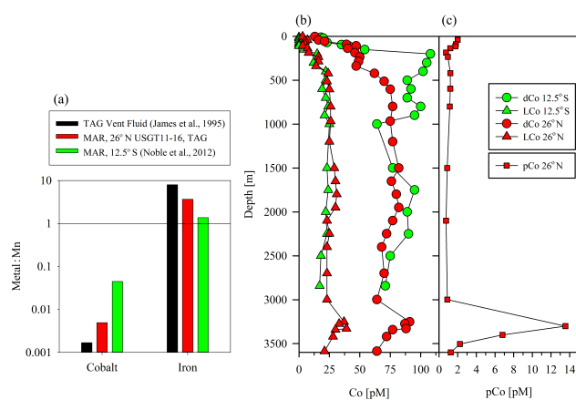
Figure 8. (a) Manganese-normalized cobalt and iron concentrations in hydrothermal fluid and above the Mid-Atlantic Ridge. Hydrothermally leached crust may reflect ratios of reducible metals that are similar to that found in crustal material. Normalized cobalt and iron values are consistent with what might be expected by dilution of hydrothermal fluids measured at TAG. This is consistent with dissolved data from above the Mid-Atlantic Ridge at 9° S as well. (b) Profiles of dissolved total and labile cobalt above the TAG hydrothermal vent and above the Mid-Atlantic Ridge at 9° S. A slight maximum in total and labile cobalt suggests that hydrothermally released cobalt at TAG is primarily labile and that the vent may provide a small, local source of cobalt. (c) Particulate cobalt profile at TAG.
