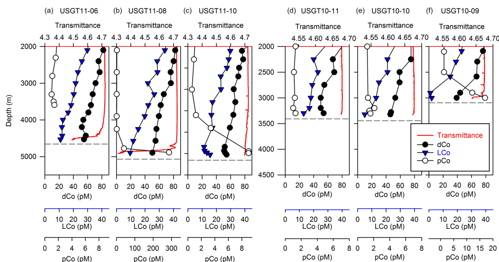
Figure 9. Along the margins, nepheloid layers have differing effects on the dissolved cobalt concentration and composition. Thick and large nepheloid layers along the western margin ( a , b , c ) appear to have small or insignificant effects on the dissolved and labile cobalt profiles, while a moderate nepheloid layer along the eastern margin at USGT10-09 ( f ) appears to have a strong scavenging effect on the dissolved cobalt. Labile cobalt in the deepest samples here were below the detection limit. The differences in the effect of nepheloid layers on the dissolved cobalt concentrations demonstrates chemical diversity in the dissolved–particulate phase interactions.
