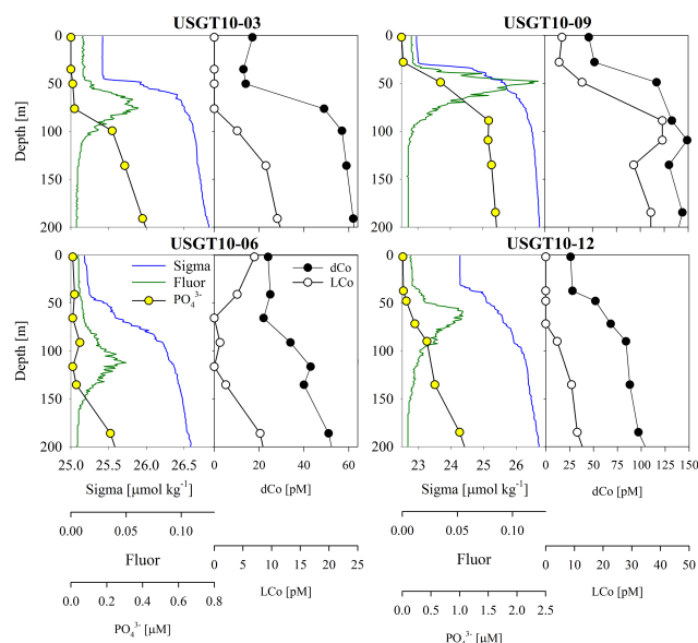
Figure 12. In the upper water column, labile cobalt is often drawn down above and within the chlorophyll maximum, following the phosphocline. The total cobaltcline appears to be more closely associated with mixed layer depth. Comparing stations that do and do not experience upwelling show that biological processes are capable of complexing labile cobalt at a rate faster than upward mixing. This is seen by comparing USGT10-03 (oligotrophic waters) to stations USGT10-12 (within the Mauritanian Upwelling). At both locations, labile cobalt is drawn down below detection into the chlorophyll maximum. Station USGT10-03 has a smaller deep inventory of cobalt ( \sim 50 pM at the chlorophyll max, increasing to \sim 60 at 200 m). Station USGT10-12 has a much larger deep inventory of cobalt ( \sim 70 pM at the chlorophyll max, increasing to \sim 100 pM at 200 m).
