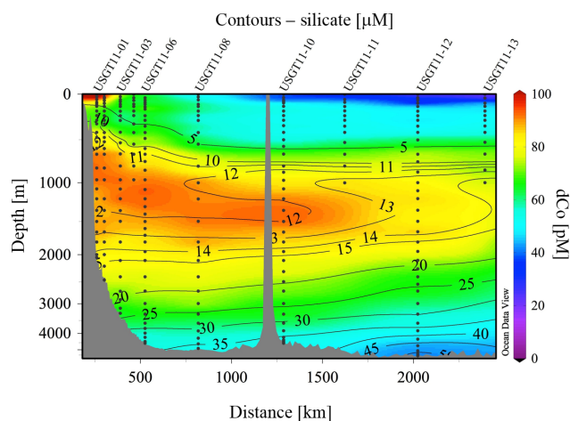
Figure 5. Section of dissolved cobalt and dissolved silicate along the western margin of the North Atlantic (Line W). Upper Labrador Sea Water, identified generally between 700 and 1500 m depth by OMPA (Jenkins et al., 2015) carries elevated concentrations of cobalt and is depleted in silicate.
