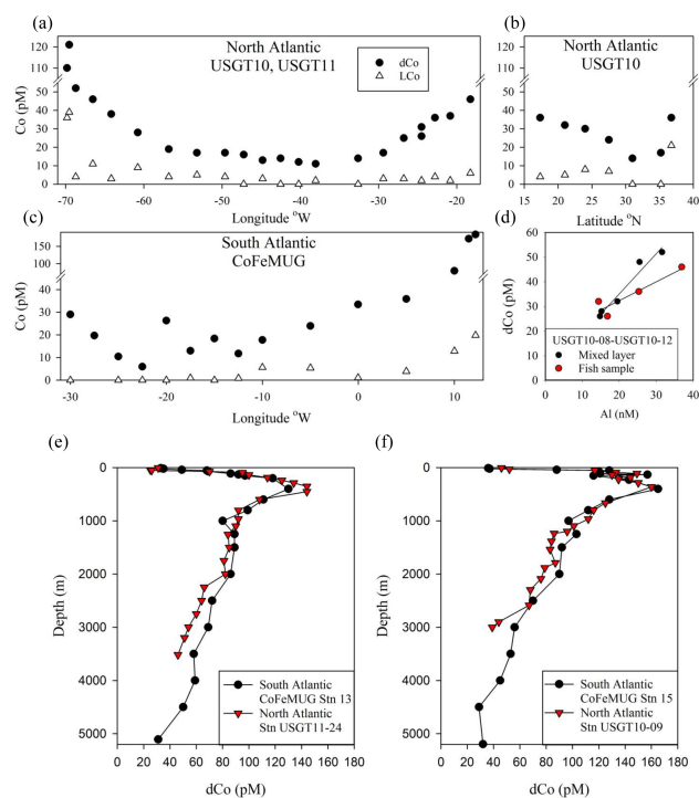
Figure 7. Surface transects of surface fish samples ( \sim 2 m) from (a–b) the North Atlantic zonal section USGT10 and USGT11, and (c) the shallowest samples ( \sim 5 – 10 m) from the South Atlantic zonal section CoFeMUG (Noble et al., 2012). (d) Relationships between dCo : dAl and correlations for northeast Atlantic stations USGT10-08 to USGT10-12. (e–f) Comparison of vertical profiles of dCo between the North and South Atlantic zonal sections near the African coast. Distances of stations to the African coastline were \sim 530 km for TENATSO (USGT11-24) and 210 km from USGT10-09 in the North Atlantic, and 1300 km for Station 13 and 790 km for Station 15 from the CoFeMUG Expedition in the South Atlantic.
