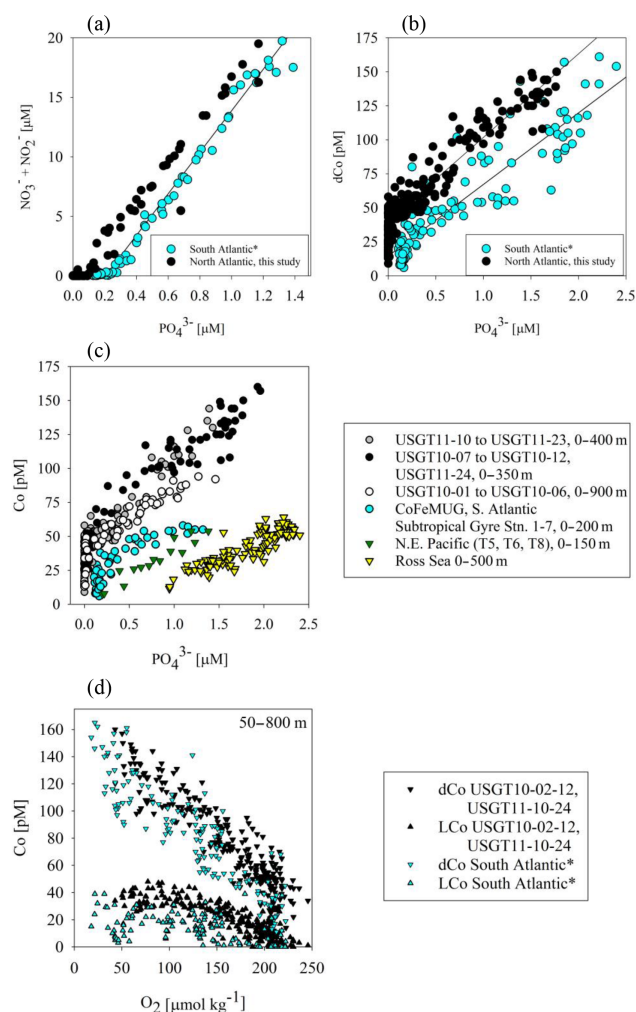
Figure 10. Aggregate nutrient stoichiometries between the North Atlantic and the South Atlantic studies. Basin offsets were observed in comparisons between (a) nitrate and phosphate (linear regression for South Atlantic with a slope of 17.4, r^2 of 0.995) and (b) cobalt and phosphate concentrations in the upper water column of the North and South Atlantic zonal sections (North Atlantic stations, 2–400 m, linear regression depths include 54–300 m, with a slope of 61.4, r^2 of 0.90; South Atlantic stations 1–19, 54–300 m, same depths for linear regression, slope of 52.6, and r^2 of 0.83). (c) Different slopes and intercepts are observed across many regions of the world oceans that have been studied in the literature (Martin et al., 1989; Noble et al., 2012; Saito et al., 2010). (d) Linear relationships occur between cobalt and oxygen for USGT10, USGT11, and for previous work done in the South Atlantic. *Data from Noble et al. 2012.
