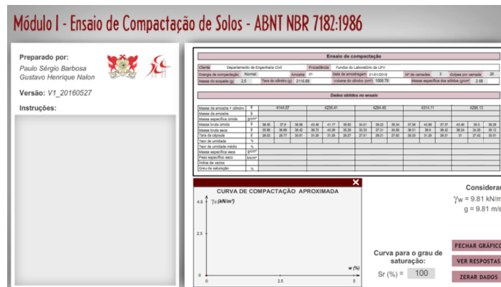
Figure 1: Central and lateral screen areas for the soil compaction test’s module.
