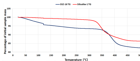
FIGURE 10. Examples of TG curves - percentage of the sample mass based on initial mass vs. temperature; red - silicalite-1 templated with \text{TPA}^+ ; blue - SSZ-16 templated with \text{Et}_6\text{-diquat-5}^{2+} .
