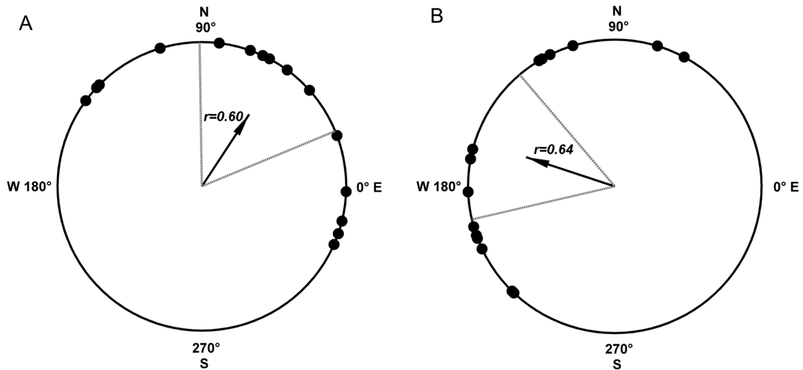
Fig. 3. The flight orientation deflection after magnetized by 1.8 T static magnetic field. (A) Armyworm moths in the geomagnetic field commonly oriented with the mean direction of 56.7^\circ , and the lower / upper 95% confidence limit was 22.5^\circ/90.9^\circ (Rayleigh test, P<0.05 ). (B) Armyworm moths magnetized by 1.8 T high stable magnetic field commonly oriented with the mean direction of 161.7^\circ with the 95% confidence intervals of 130.4^\circ - 193.0^\circ .
