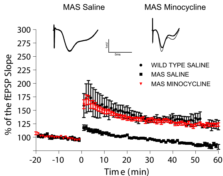
Figure 1 Minocycline restores the synaptic plasticity defect in the AS mouse model. 3-month-old UBE3A maternal deficient (AS) mice show increase in long-term potentiation (LTP) after 21 days of treatment with minocycline. Field extracellular postsynaptic potentials (fEPSPs) were recorded and their slopes are conveyed as a percentage of the pre-theta burst stimulation (TBS) baseline. Representative traces before (bold) and 30 minutes after TBS are shown for saline treated (control) and minocycline treated AS mice.
