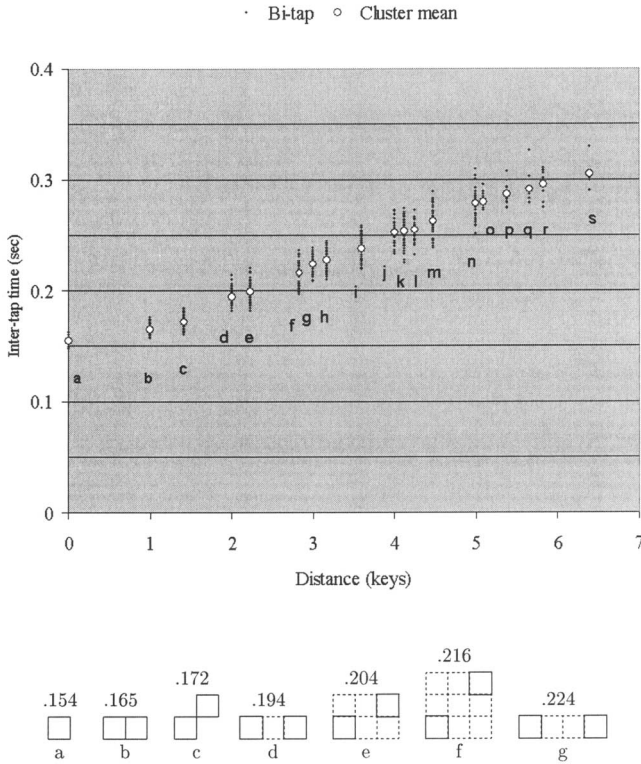
Figure 5. (Upper) Time-distance scatter plot of the 900 bi-tap times in the empirical bi-tap table (Figure 4), the aggregated results from our experiments. (Lower) Chart illustrating a typical relation (modulo rotation and reflection) between keys of bi-taps in clusters a to g of the plot. For example, cluster a consists of double-taps on the same key (30 data points), cluster b consists of bi-taps between immediate neighbors (98 data points: 24<, 24@, 25<, 25@), cluster c consists of bi-taps between diagonal neighbors (80 data points: 20™, 20(, 20@, 20Σ), and so on. Cluster means are quoted above the corresponding pictures (.154, .165, ...).
