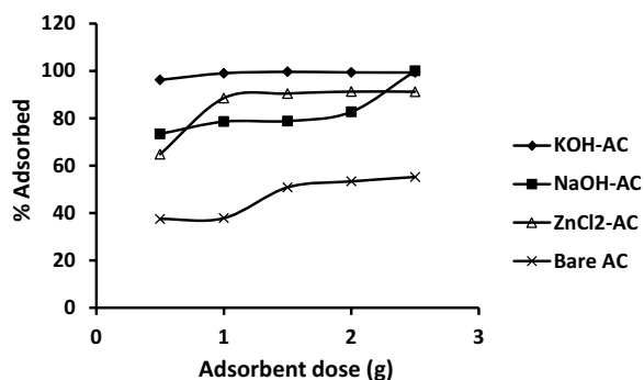
Fig. 3 Effect of adsorbent dosage on the adsorption of Cd 2+ by ZnCl 2 , KOH and NaOH AC, and the regular activated doum palm powder
