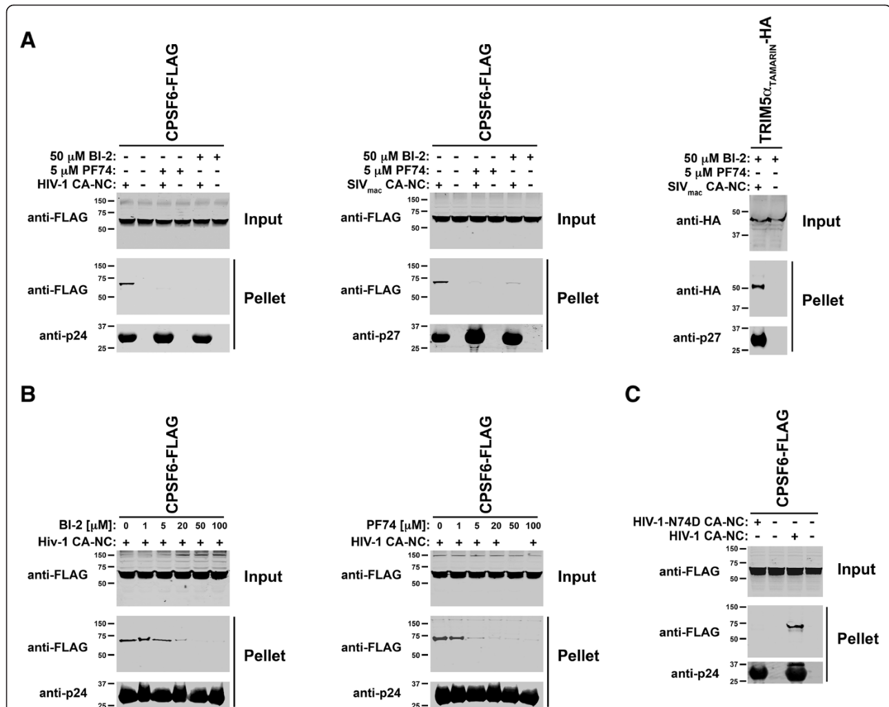
Figure 3 BI-2 prevents the binding of the cellular factor CPSF6 to HIV-1 CA-NC complexes. (A) The ability of CPSF6 to bind in vitro assembled HIV-1 CA-NC complexes in the presence of BI-2 was analyzed as previously described [22]. Briefly, extracts of 293 T cells transiently transfected with a CPSF6-FLAG construct (Input) were incubated with in vitro assembled HIV-1 or SIV mac CA-NC complexes in the presence BI-2 for 1 h. Subsequently, extracts were applied onto 70% sucrose cushion and centrifuged, and the pelleted fraction was collected (Pellet). Input and Pellet fractions were analyzed using anti-FLAG and anti-p24 antibodies. As control, the binding of CPSF6 to in vitro assembled HIV-1 CA-NC complexes was studied in the presence of PF74. Similar results were obtained in three independent experiments and a representative experiments is shown. To control for the bona fide origin of in vitro assembled SIV mac CA-NC complexes, we tested the ability of TRIM5 \alpha protein from Tamarin monkeys tagged with an HA epitope (TRIM5 \alpha_{Tamarin} -HA) to bind SIV mac capsid. (B) The ability of CPSF6 to bind in vitro assembled HIV-1 CA-NC complexes in the presence of increasing concentrations of BI-2 was analyzed (left panel). As a control, similar experiments were performed using increasing concentrations of PF74 (right panel). Similar results were obtained in three independent experiments and a representative experiments is shown. (C) To show that the interaction of CPSF6 with in vitro assembled HIV-1 CA-NC complexes is only dependent upon the capsid protein, we tested the ability of CPSF6 to bind in vitro assembled HIV-1 CA-NC complexes bearing the change N74D. Similar results were obtained in three independent experiments and a representative experiments is shown.
