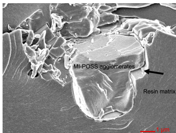
Figure 4 High magnification scanning electron microscope micrographs of MI10.
