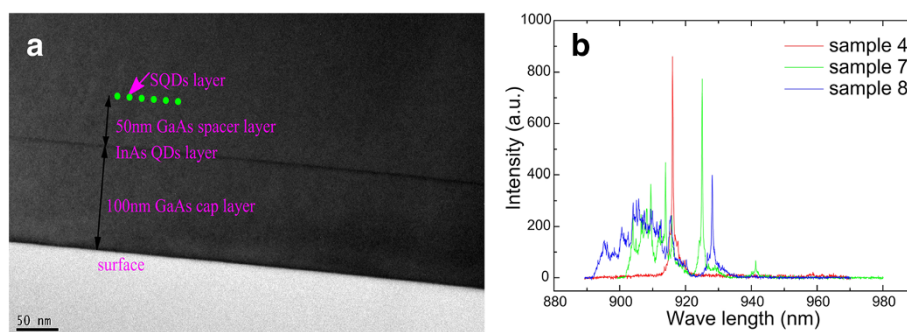
Figure 6 TEM and micro-PL. (a) TEM of sample 10. (b) Micro-PL of samples 4, 7, and 8 annealed respectively at 650°C, 630°C, and 620°C.
