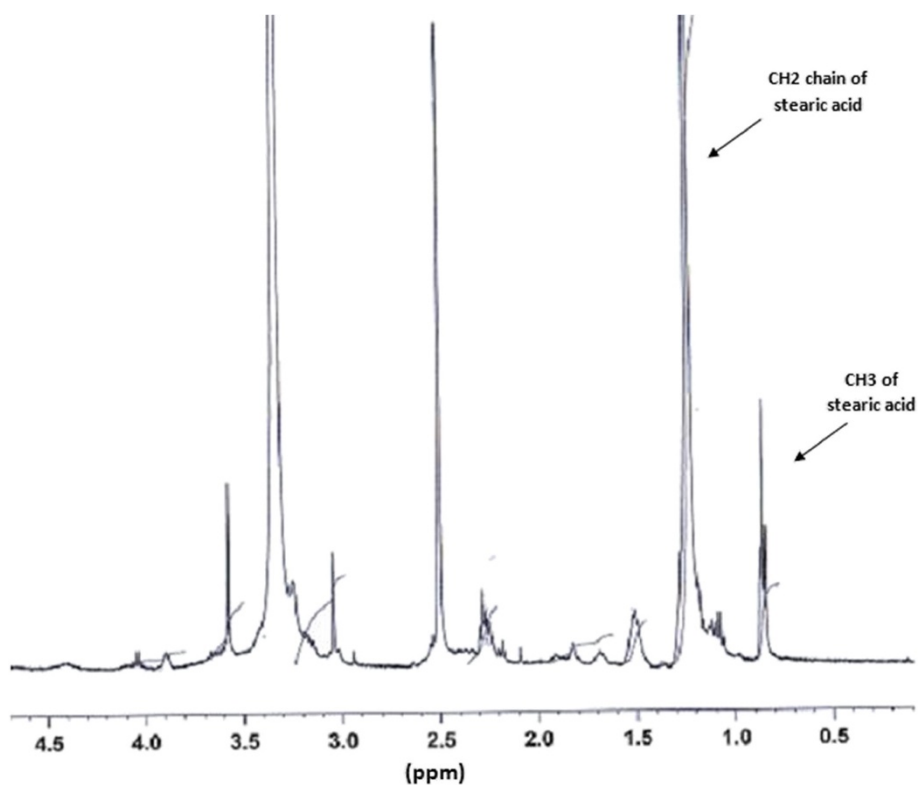
Figure 3 HNMR spectra of depolymerized chitosan grafted to stearic acid in DMSO-d6.
