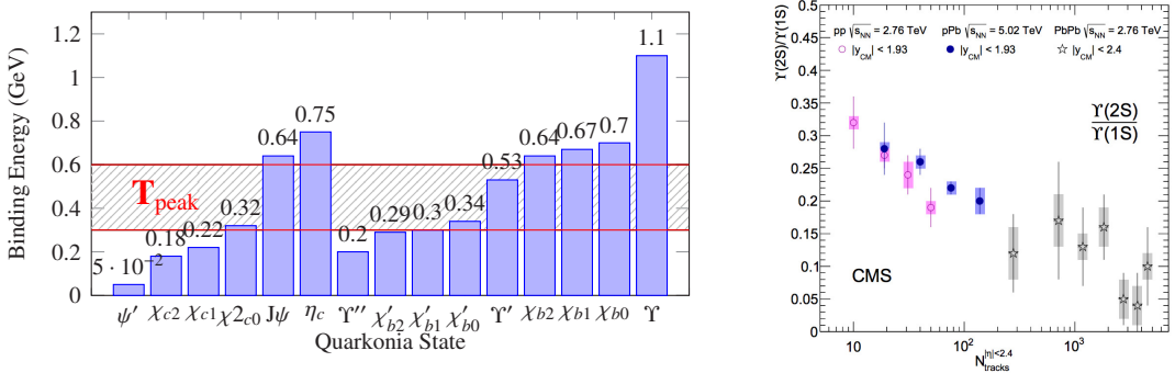
Figure 3: (left) Binding energy of several quarkonium states in vacuum [31] along with an estimation for the quark-gluon plasma peak temperature at RHIC [32] as hashed area. (right) Relative Y(2S)/Y(1S) yields versus particle multiplicity in p+p , p+Pb and Pb+Pb collisions measured by CMS [33].
