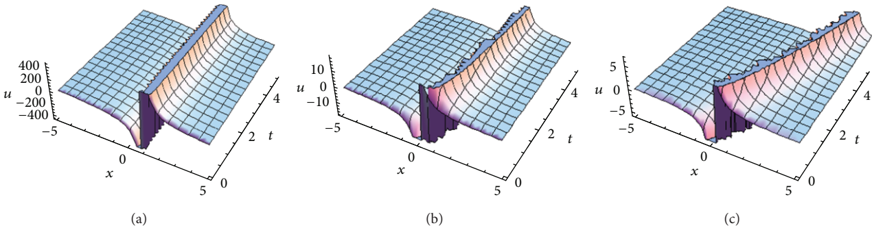
FIGURE 3: Graphics of the solution equation (52) corresponding to the values \alpha = \beta = 0.01 , \alpha = \beta = 0.25 , and \alpha = \beta = 0.75 from left to right when k = a_2 = b_0 = 0.1, -5 < x < 5 , and 0 < t < 5 .
