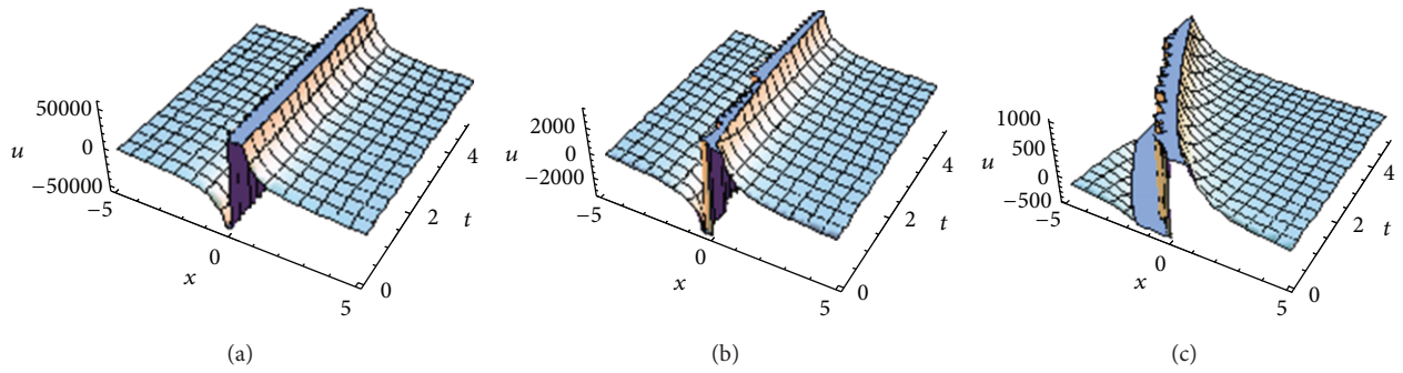
FIGURE 2: Graphics of the solution equation (40) corresponding to the values \alpha = \beta = 0.01 , \alpha = \beta = 0.25 , and \alpha = \beta = 0.75 from left to right when k = a_1 = b_0 = b_1 = \gamma = 0.01, -5 < x < 5 , and 0 < t < 5 .
