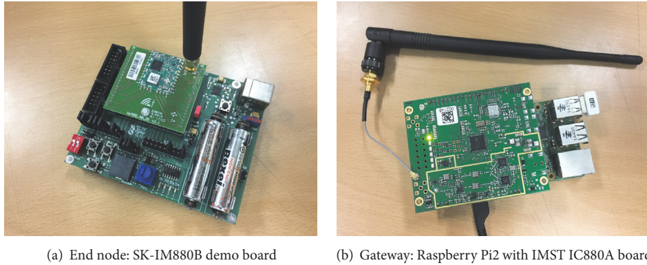
FIGURE 6: LoRaWAN devices.
