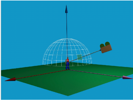
Figure 2: To create an impostor, images are computed for discrete positions of a camera around a hemisphere surrounding the avatar.
