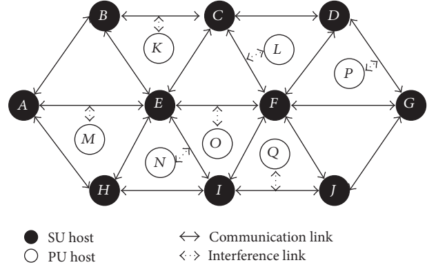
FIGURE 1: Network scenario.
