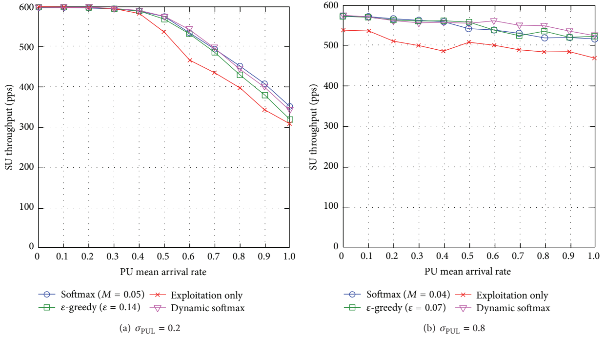
FIGURE 14: SU throughput for varying PU mean arrival rate \mu_{\text{PUL}} for different levels of standard deviation of PUL \sigma_{\text{PUL}} .
