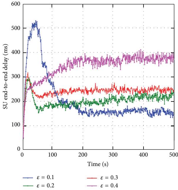
FIGURE 10: SU end-to-end delay for varying exploration probability \epsilon .
