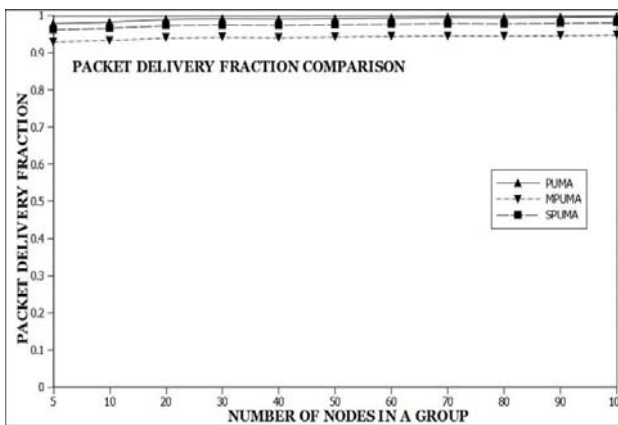
Figure 2. Packet delivery fraction of PUMA With and Without MITM Attack Vs Secure PUMA
