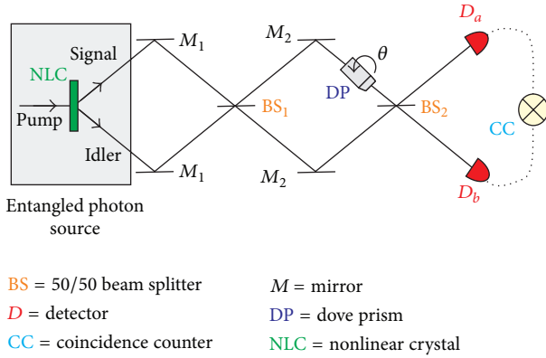
FIGURE 4: Schematic of setup for super-resolution angular displacement measurements using entangled OAM states. Spontaneous parametric downconversion in a nonlinear crystal (on the left) sends entangled photon pairs into a Mach-Zehnder interferometer (middle portion) which contains a Dove prism in one arm. On the right, photodetectors are connected to a coincidence circuit, so that an event is registered only when both detectors fire within a short time window.
