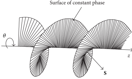
FIGURE 2: Optical wavefronts with nonzero orbital angular momentum have corkscrew-shaped wavefronts. The Poynting vector, \mathbf{S} , must be everywhere perpendicular to the wavefront, so it rotates as the wave propagates along the z -axis.
