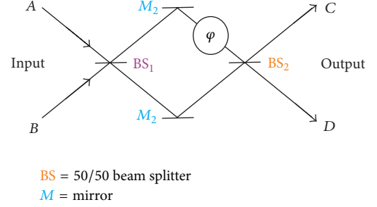
FIGURE 1: A Mach-Zehnder interferometer. Input at either of the input ports ( A or B ) has two possible ways of reaching the final beam splitter, BS_2 . Along the upper path, a phase shift of \phi is added. The second beam splitter makes it impossible to determine which path was followed simply from looking at the output at ports C and D . As a result, the amplitudes for the both possibilities must be present, leading to interference at the output ports.
