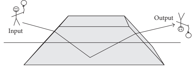
FIGURE 3: Dove prism. Total internal reflection at the horizontal surface causes images to be inverted vertically.
