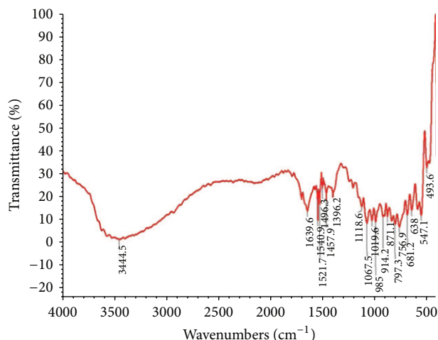
FIGURE 4: FTIR analysis of synthesized silver nanoparticles from Westiellopsis sp. (A.15). Wavenumbers \text{cm}^{-1} : 1 unit = 500 \text{cm}^{-1} ; % transmittance: 1 unit = 10% transmittance.
