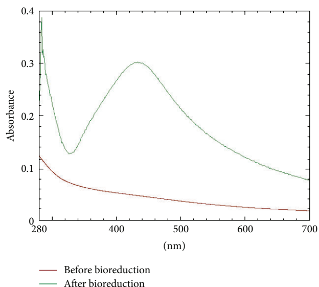
FIGURE 2: The UV/Vis absorption spectra of silver nanoparticles. nm: wavelength in nanometers (1 unit = 100 nm); Abs: absorbance (1 unit = 0.1 absorbance unit).
