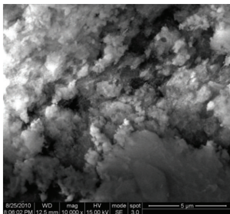
FIGURE 3: Scanning electron micrograph of silver nanoparticles. WD: working distance between the sample surface and the low portion of the lens which should be greater than 4 mm (12.5 mm); Mag: magnification at 10000x; HV: high voltage (15 kV); Mode: secondary electron (SE) mode.
