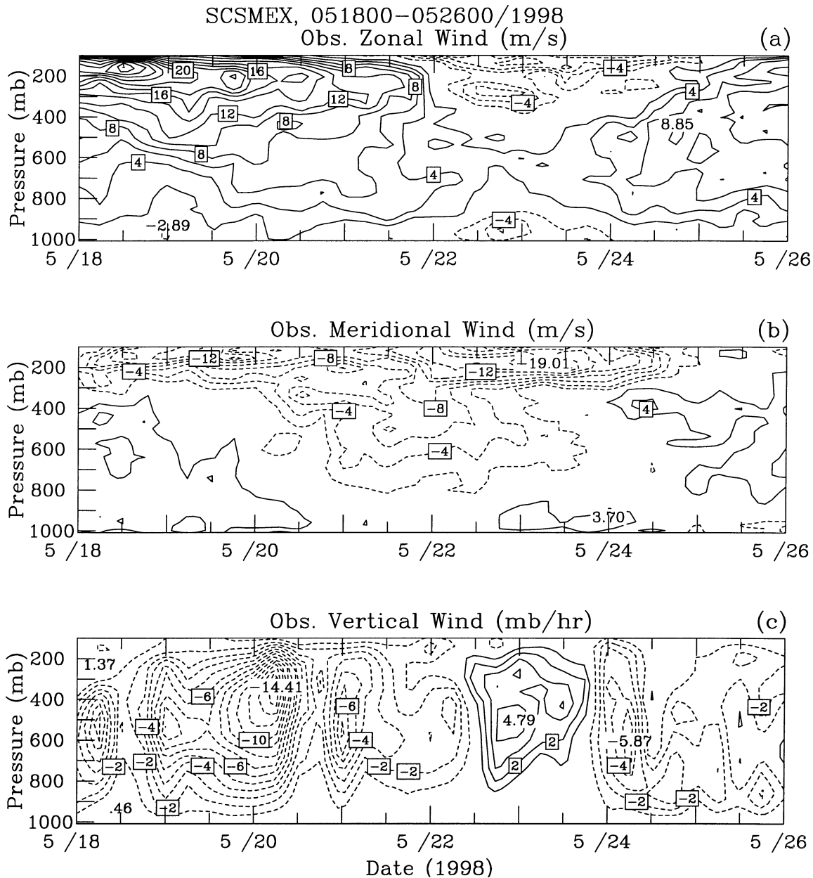
FIG. 3. Horizontally averaged mean large-scale (a) u wind ( \text{m s}^{-1} ), (b) v wind ( \text{m s}^{-1} ), and (c) w velocity ( \text{mb h}^{-1} ) for the 18–26 May 1998 period. The contour interval is 2 \text{ m s}^{-1} , 2 \text{ m s}^{-1} , and 1 \text{ mb h}^{-1} for (a), (b), and (c), respectively. (d), (e), (f) Same as (a), (b), and (c), except for the 2–11 Jun 1998 period.
