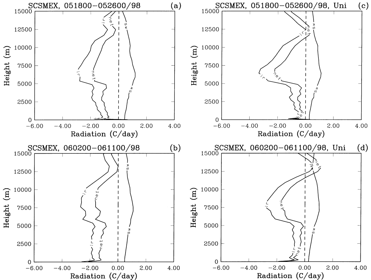
FIG. 16. Vertical profiles of time- and domain-averaged radiation (total, longwave cooling, and shortwave heating) for the (a) May and (b) Jun SCSMEX cases. (c), (d) Same as (a), (b), except for the sensitivity tests.
