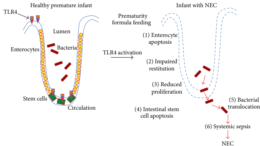
FIGURE 1: Mechanisms to explain how TLR4 activation in the premature intestinal epithelium is required in the pathogenesis of necrotizing enterocolitis. As shown, colonization of the intestine of the premature infant leads to the activation of TLR4 within the intestinal epithelium as well as on the intestinal stem cells, due in part to the elevated expression levels of TLR4 in the setting of prematurity. TLR4 activation leads to enterocyte apoptosis, impaired restitution and reduced proliferation as well as stem cell apoptosis, leading to bacterial translocation, systemic sepsis, and the development of NEC. See text for further details.
