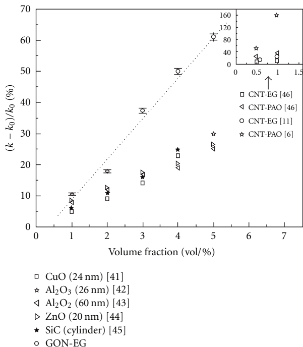
FIGURE 4: Thermal conductivity enhancement ratios of EG-based nanofluids as a function of loading. The inset shows the thermal conductivity enhancement ratios of nanofluids containing CNTs.
