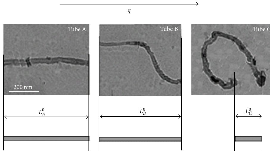
FIGURE 3: Actual nonstraight CNTs (left two) and equivalent straight thermal passages (right).
