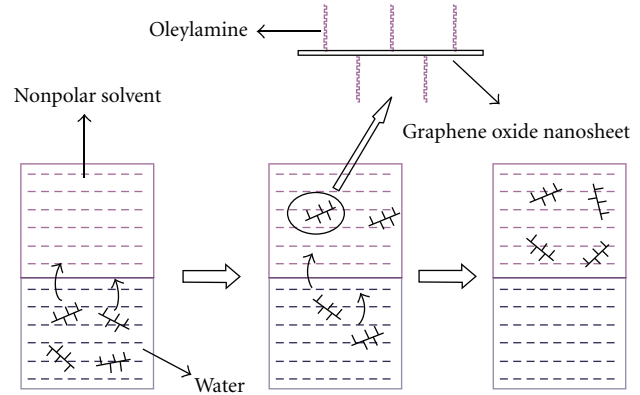
FIGURE 1: Schematic illustration of the phase transfer process.
