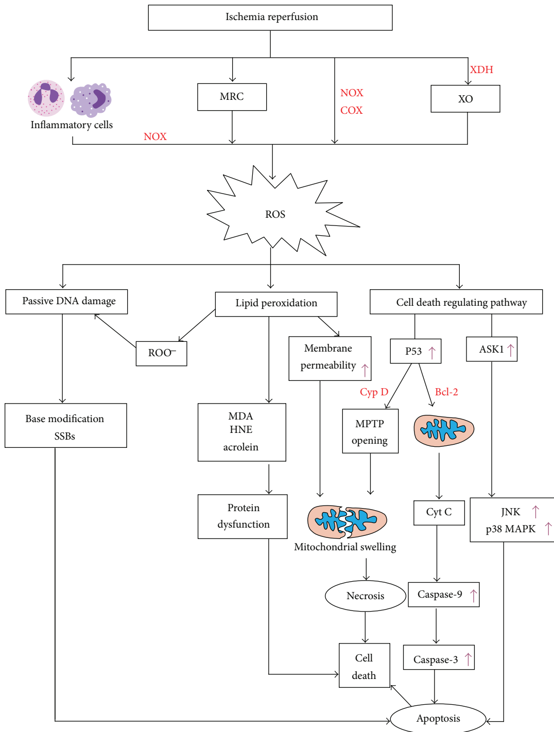
FIGURE 1: ROS damage in ischemia-reperfusion injury. First, ROS-generated pathways: MRC; NOX; COX-2; XO. ROS react with DNA and then cause passive DNA damage leading to base modification and SSBs which induce to apoptosis. Reaction of \text{OH}^- with unsaturated fatty acids generates \text{ROO}^- which may also cause passive DNA damage. The products of lipid peroxidation such as MDA, HNE, and acrolein can lead to protein dysfunction. Besides, lipid peroxidation increases membrane permeability inducing to mitochondrial swelling. P53 activated by ROS can also cause mitochondrial swelling by MPTP opening via reaction of P53 with Cyp D. P53 induces Cyt C released from mitochondria by reacting with Bcl-2 family proteins and subsequently leads to caspase cascade causing apoptosis. What is more, ROS can activate JNK and p38 MAPK pathways which are activated by ASK1 and lead to apoptosis. MRC: mitochondrial respiratory chain; NOX: NADPH oxidases; COX-2: cyclooxygenase-2; XDH: xanthine dehydrogenase; XO: xanthine oxidase; ROS: reactive oxygen species; SSBs: single-strand breaks; \text{ROO}^- : peroxy radical; MDA: malondialdehyde; HNE: 4-hydroxynonenal; Cyp D: cyclophilin D; Cyt C: cytochrome C; MPTP: mitochondrial permeability transition pore; ASK1: apoptosis signal-regulating kinase 1; JNK: c-Jun NH2-terminal kinase; p38 MAPK: p38 mitogen-activated protein kinase. “↑” demonstrates events that are increased or enhanced.
