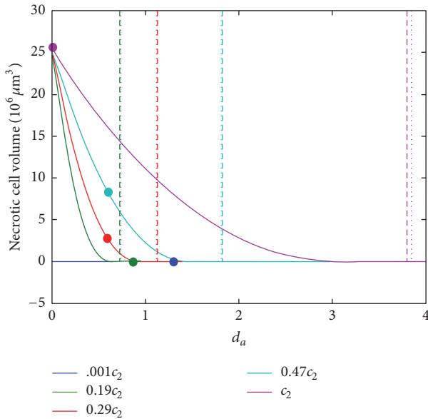
FIGURE 7: Bifurcation diagram for equilibrium of necrotic cells in spheroid model. Each line represents the equilibrium volume of cells at a different treatment intensity c_{2,\text{new}} , as a function of d_a , in units of 10^6 \mu\text{m}^3 . Filled circles denote the equilibria using the fitted pair of parameters (c_{2,\text{new}}, d_{a,\text{new}}) in Table 2 and Figure 2 (control, c_2 = 3.85 , d_a = 0 ), ( 2 \mu\text{M} , c_{2,\text{new}} = 0.47c_2 , d_{a,\text{new}} = 0.60 ), ( 4 \mu\text{M} , c_{2,\text{new}} = 0.29c_2 , d_{a,\text{new}} = .59 ), ( 8 \mu\text{M} , c_{2,\text{new}} = 0.19c_2 , d_{a,\text{new}} = .87 ), and ( 12 \mu\text{M} , c_{2,\text{new}} = 0.001c_2 , d_{a,\text{new}} = 1.3 ). Vertical lines denote critical values for the monolayer model ( d_a = c_2 ). At values of d_a below these critical values the monolayer grows exponentially. For values higher than this it declines exponentially. Diagrams for the proliferating and quiescent compartments (omitted here) are similar to this diagram. Note that equilibrium values for all spheroid compartments drop to near zero before the critical value for the monolayer model.
