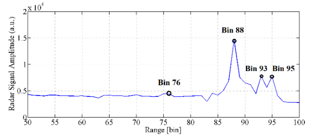
Fig. 6 Range profile and bin identification.
