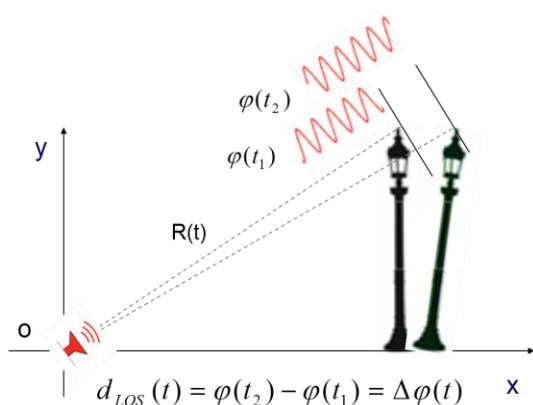
Fig. 1. A scheme of the working principle. d_{LOS} is the projection of the displacement along the radar line of site.
