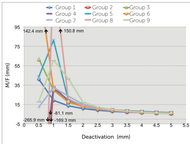
Figure 6 - Chart depicting the average M/F ratios produced during deactivation from 5 to 0.5mm for the groups tested.
