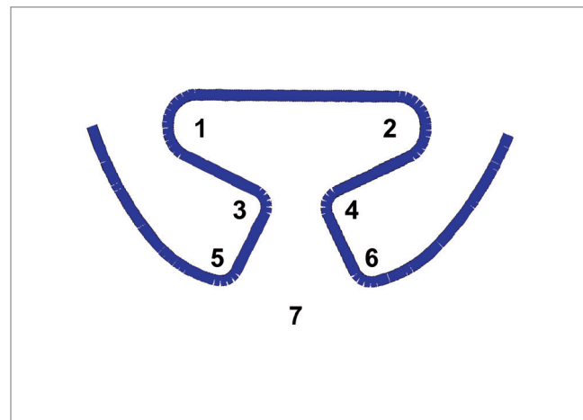
Figure 7 - TLSs structural angles measured for finding the deformation location. The angle 7 is formed by the intersection of horizontal extremities of the TLS.
