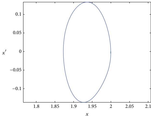
FIGURE 2: Numerical simulation for e(t) = 0.03 \times (\sin(2\pi t) - 0.179025044320086) .
