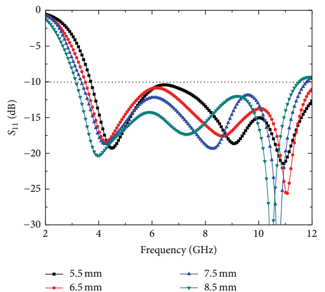
FIGURE 3: Simulated S_{11} of the single UWB antenna without EBG structures for different parameters of R_{patch} .
