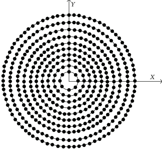
FIGURE 2: Ten-ring concentric circular ring array of isotropic antennas.
