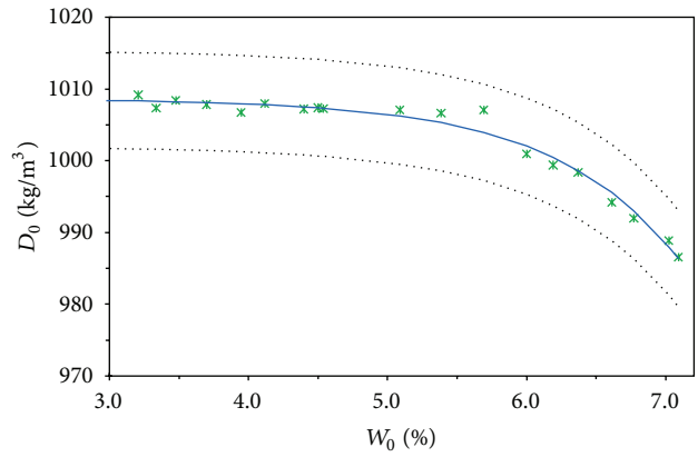
FIGURE 6: Fill density ( D_0 ) as a function of the powder moisture content ( W_0 ) with CI_{95\%} .
