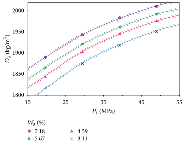
FIGURE 8: Dry bulk density ( D_3 ) as a function of the compaction pressure ( P_1 ) and powder moisture content ( W_0 ) with CI_{95\%} (dotted lines).
