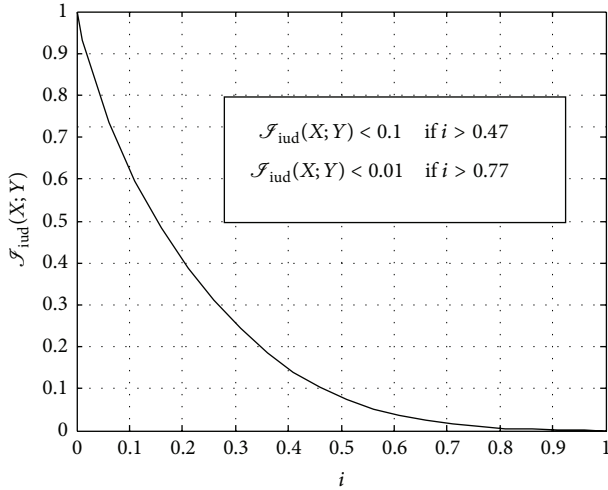
FIGURE 2: Information rate \mathcal{F}_{\text{iud}}(X; Y) as a function of insertion probability i .
