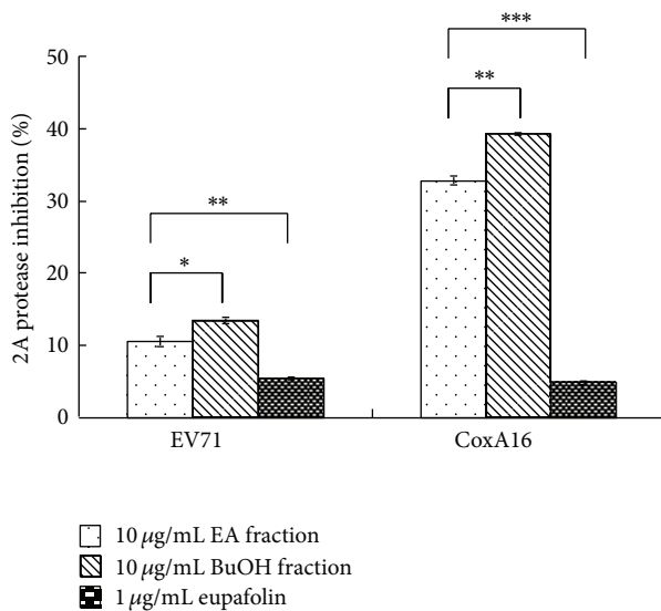
FIGURE 8: Inhibitory effect of eupafolin, EA, and BuOH fractions on viral 2A protease activity in cell-based FRET assay. HeLa-G2AwtR cells expressed 2A-cleavage motif in FRET probes were infected with EV71 or CVA16 at a MOI of 1, coexistent with treatment of eupafolin, EA, and BuOH fractions. Cells harvested 48 postinfection were subjected to measurement by a fluorescent-plate reader with excitation wavelength at 390/20 nm and emission wavelength at 510/10 nm (for GFP + ) or 590/14 nm (for DsRed2). Inhibitory activity was calculated as FRET ratio, that is, intensity of emission at 590/14 nm divided by that at 510/10 nm. * P value < 0.05; ** P value < 0.01; *** P value < 0.001 by Scheffé's test.
