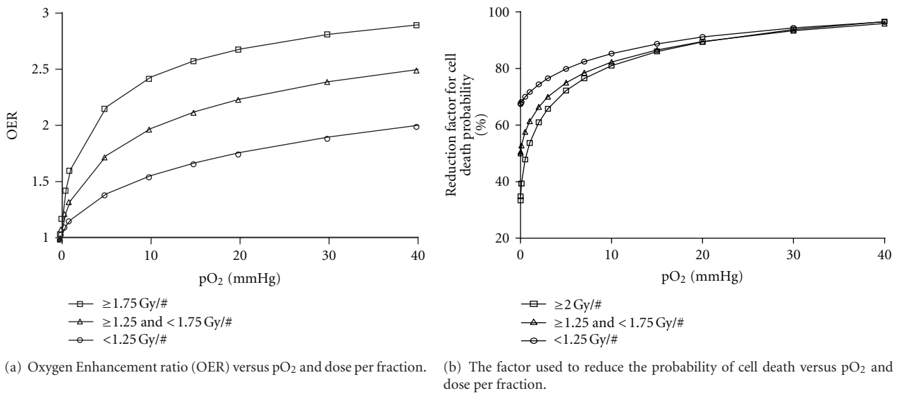
FIGURE 2: (a) Oxygen Enhancement Ratio (OER) curves implemented in the model for adjusting the radiosensitivity of cells during radiotherapy, based on cellular pO 2 and dose per fraction, and (b) conversion of the OER curves into a probability of cell death factor, through OER curve normalisation.
