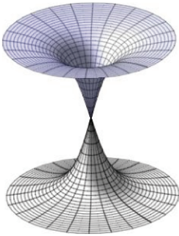
FIGURE 2: Wormhole. Shown is the embedding diagram for the two D3 -branes, D3_1 and D3_2 , with azimuthal angle suppressed. The domain of the radial coordinate, r , is 0 \leq r \leq 15L_d , and the range of the embedding coordinate x^4 is -.45L_{D3} \leq x^4 \leq +.45L_{D3} .
