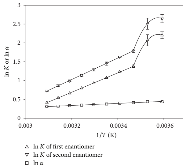
FIGURE 2: Van't Hoff plots of K and \alpha of imazamox at range of 5–50°C with 60/40 mobile phase.
