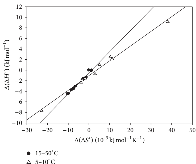
FIGURE 3: Enthalpy-entropy compensation plot of \Delta(\Delta H^\circ) versus \Delta(\Delta S^\circ) at 5–10°C and 15–50°C.
