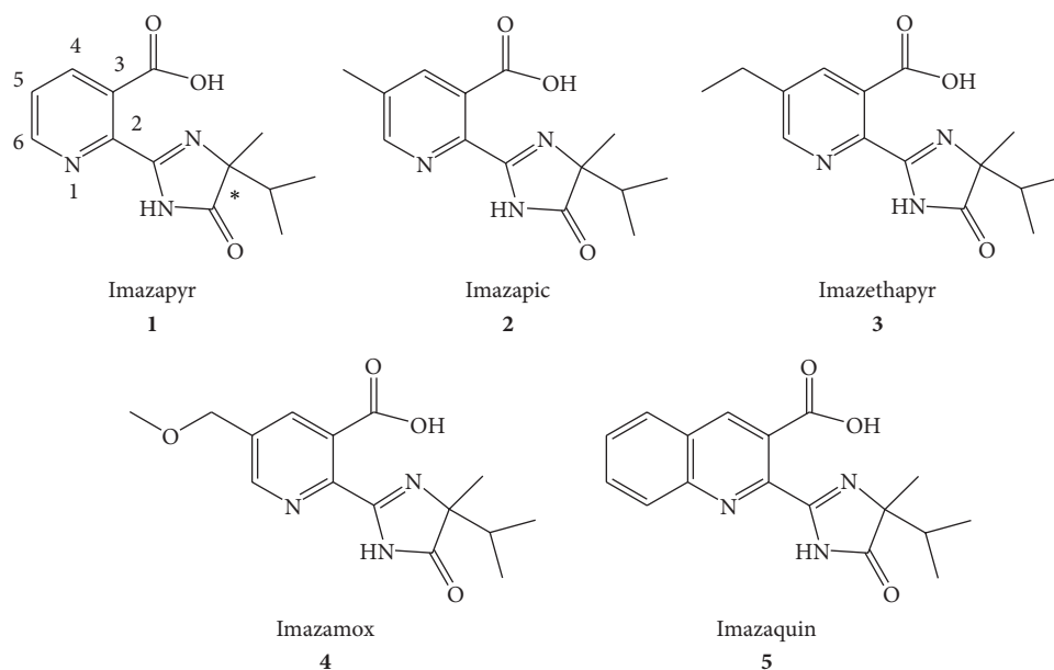
FIGURE 1: Structures of the imidazolinone herbicide.
