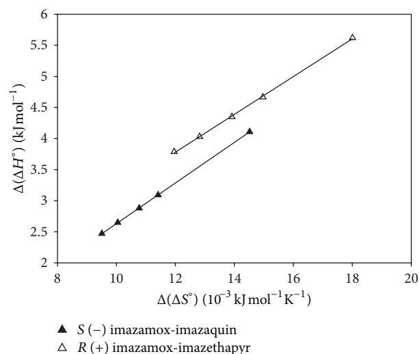
FIGURE 4: Enthalpy-entropy compensation of group selectivity for mobile phase composition.
