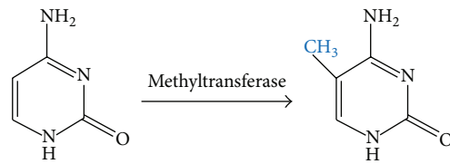
FIGURE 1: Methylation of cytosine in carbon 5.
